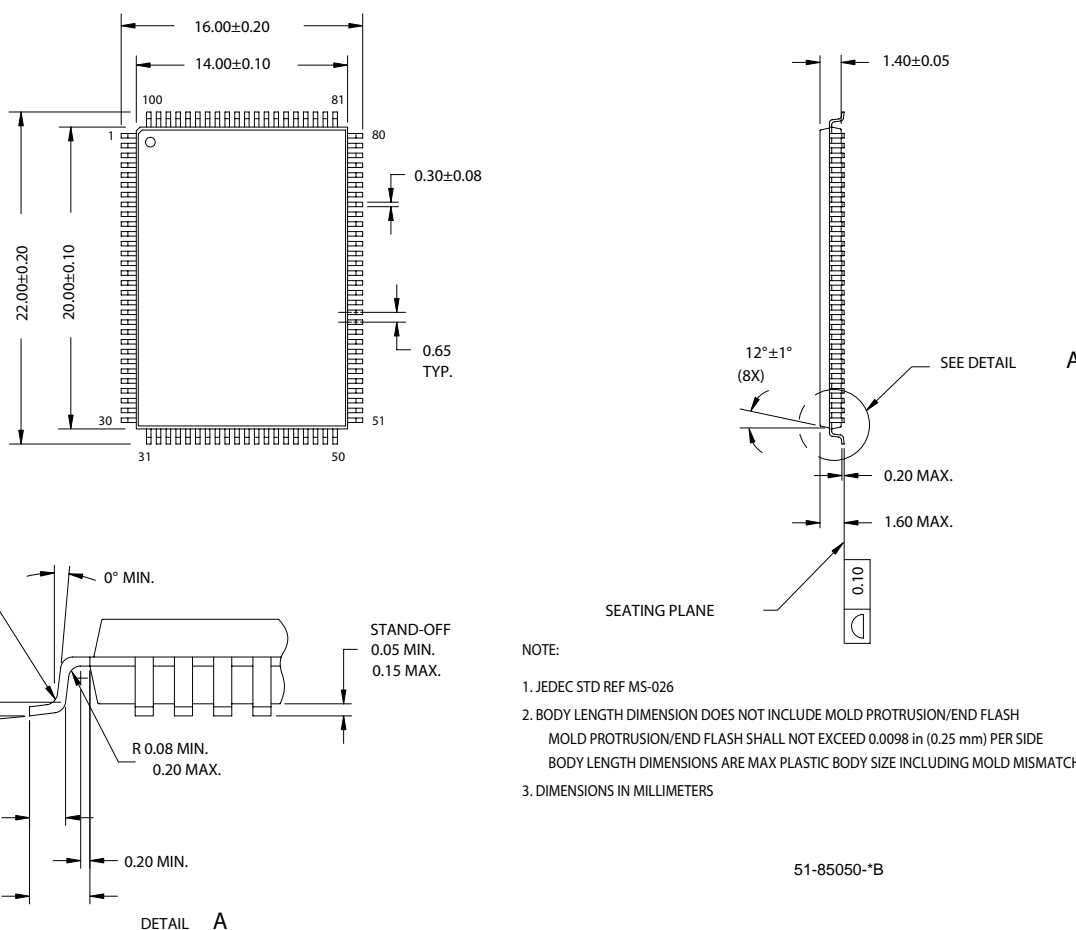
100-Pin Thin Plastic Quad Flatpack (14 x 20 x 1.4 mm) (51-85050)
