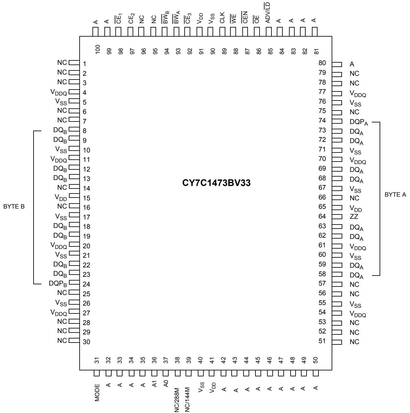
CY7C1473BV33 (4 M × 18)
