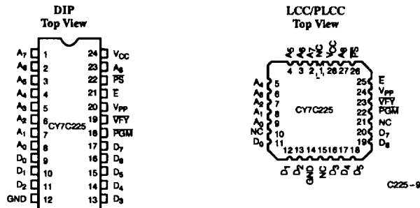
Figure 1. Programming Pinouts
