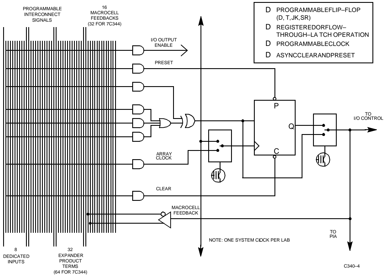
Figure 4. Macrocell Block Diagram
