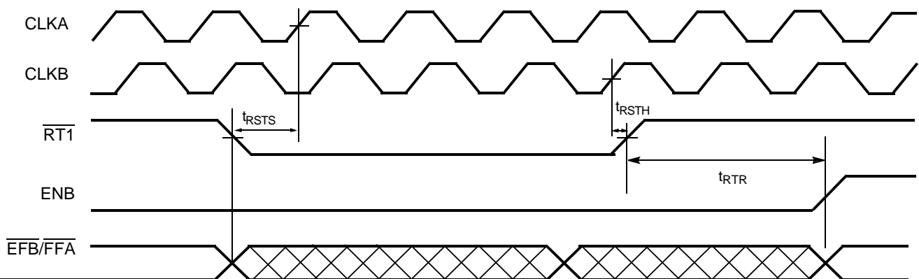
FIFO1 Retransmit Timing [50,51,52,53,54]
