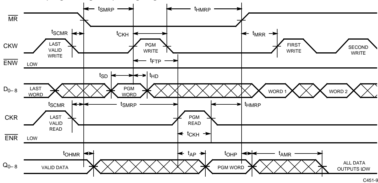
Master Reset (Programming Mode with Free-Running Clocks) Timing Diagram [20,21]
