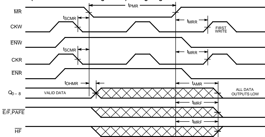
Master Reset (Default with Free-Running Clocks) Timing Diagram [18,19,20,21]
