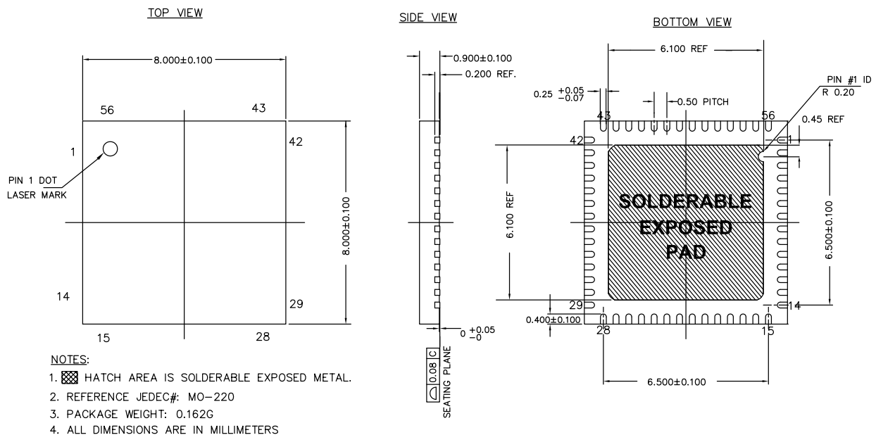
Figure 8. 56-pin Sawn QFN (8 × 8 × 1.0 mm)
