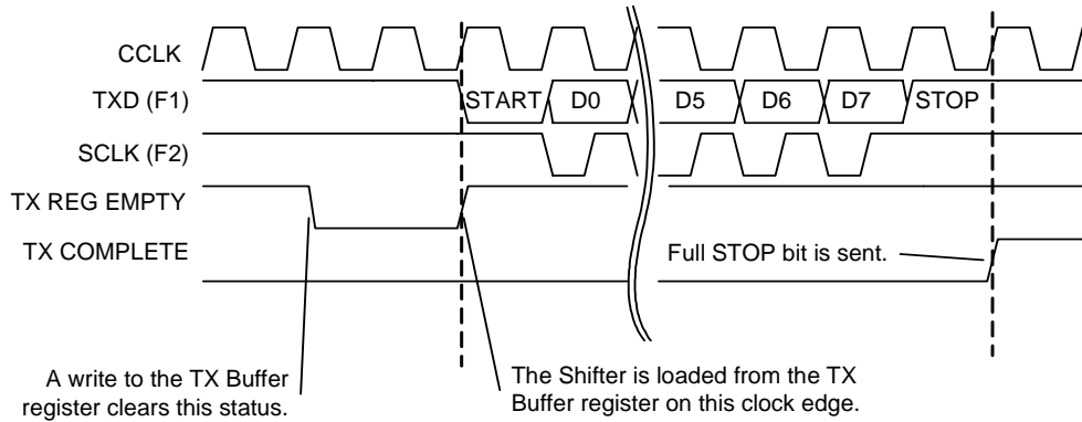
Figure 17-25. Status Timing for the Transmitter
