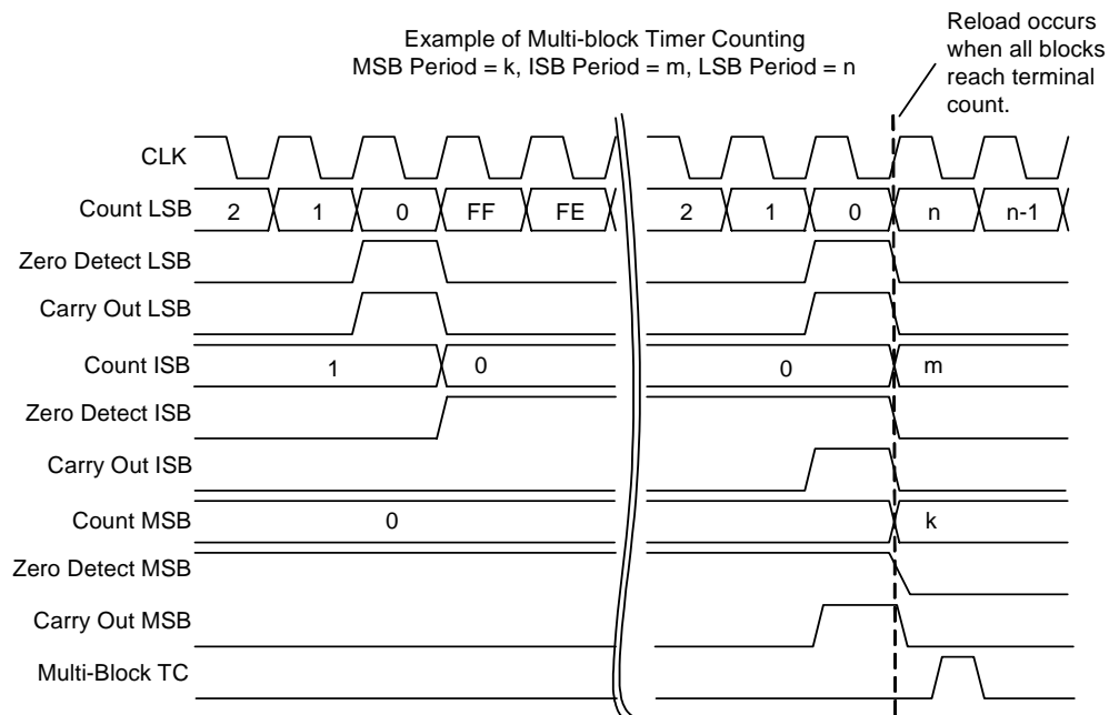
Figure 17-6. Multi-Block Timing
