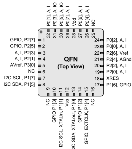
Figure 5. CY8C23533 32-Pin PSoC Device
