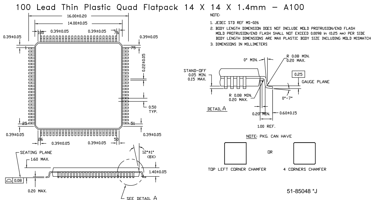
Figure 26. 100-pin TQFP (14 × 14 × 1.4 mm) Package Outline, 51-85048
