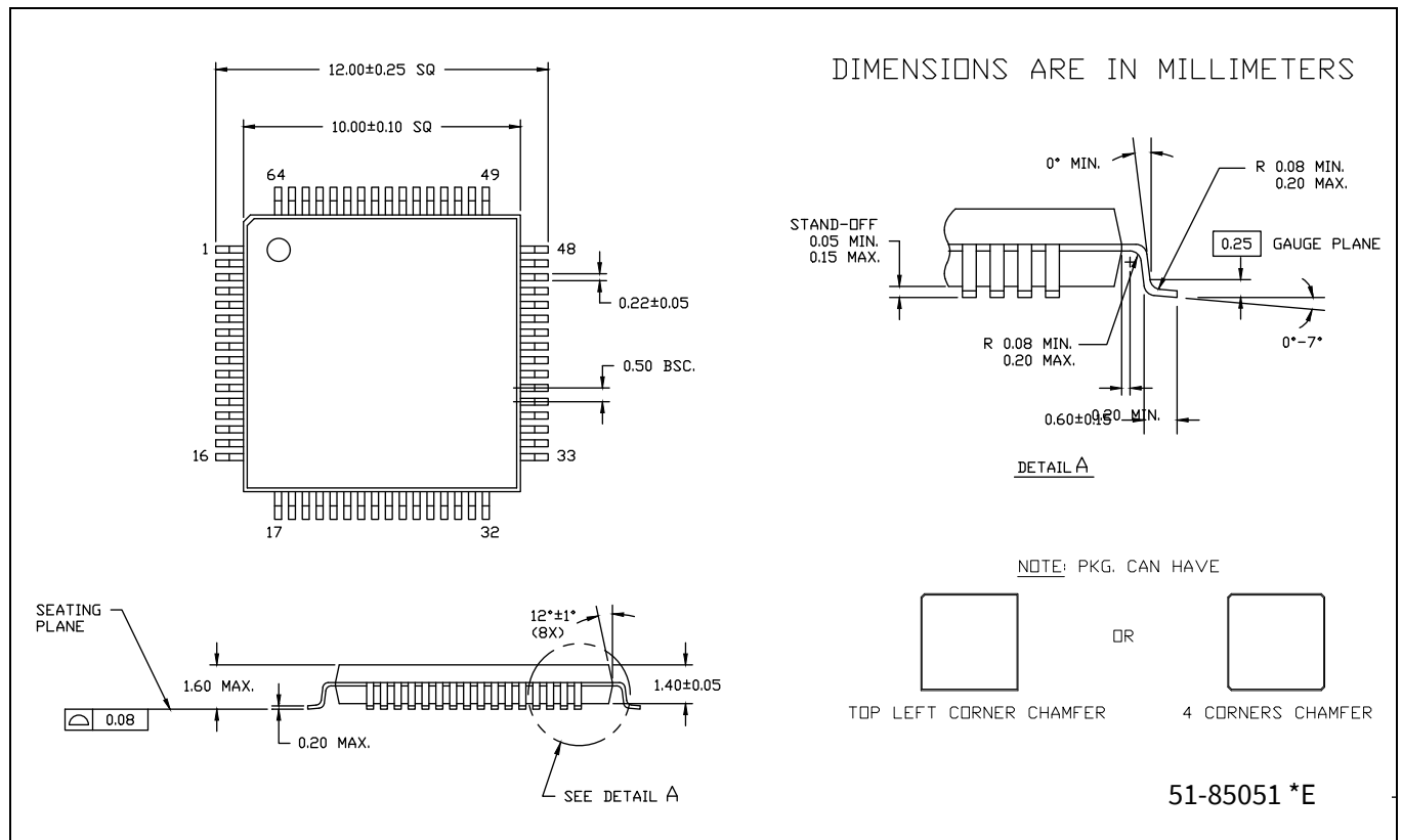
Figure 9 64LD TQFP (10 × 10 × 1.4 mm) A64SB (PG-TQFP-64) package outline
