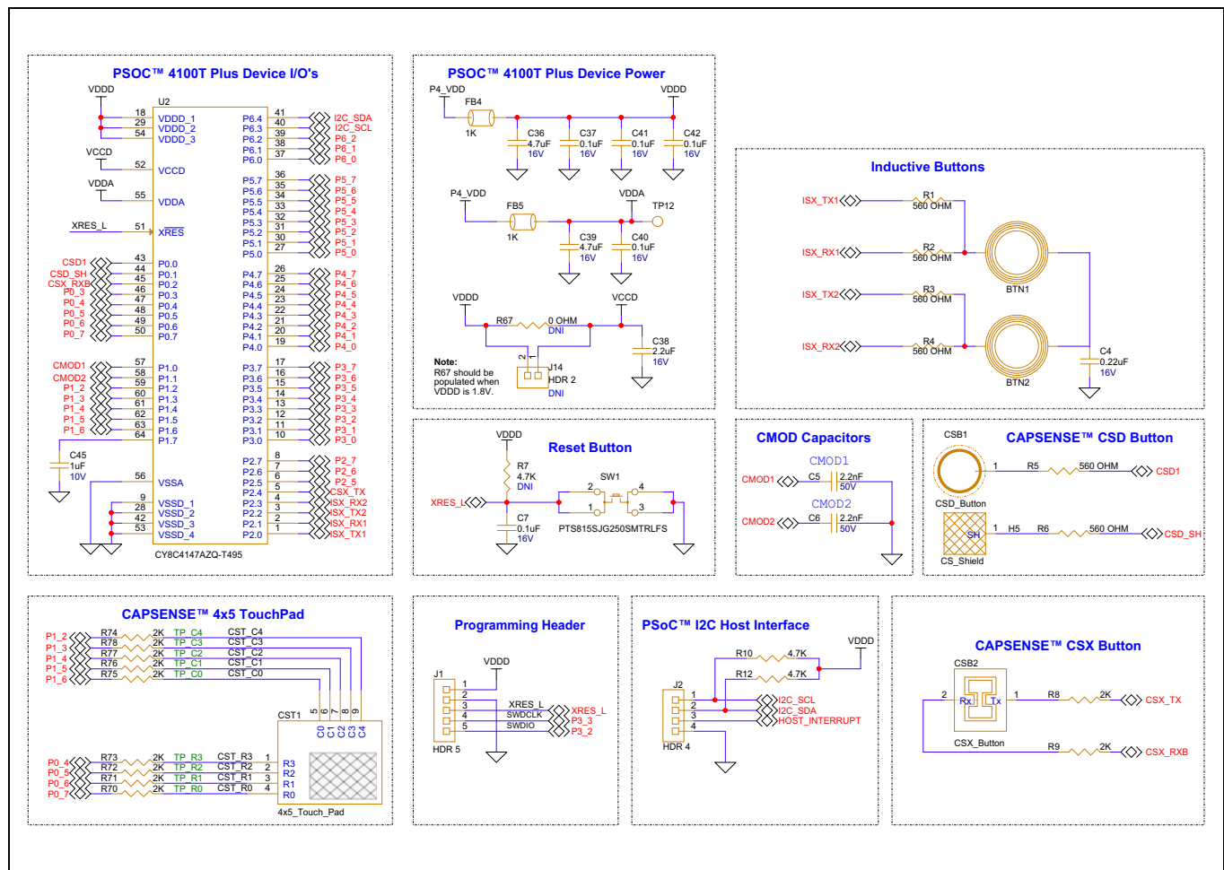
Figure 5 Application example schematic
