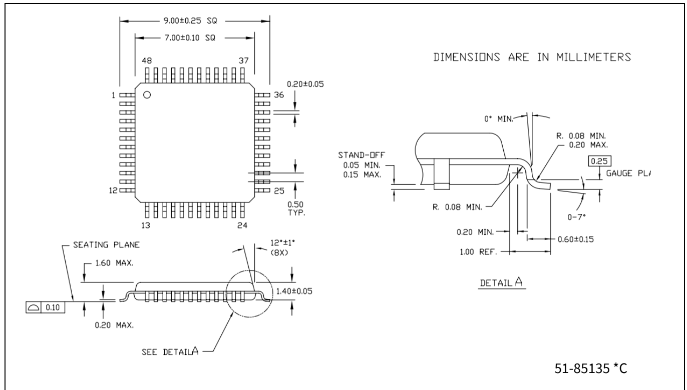
Figure 7 48LD TQFP (7 × 7 × 1.4 mm) A48 (PG-TQFP-48) package outline
