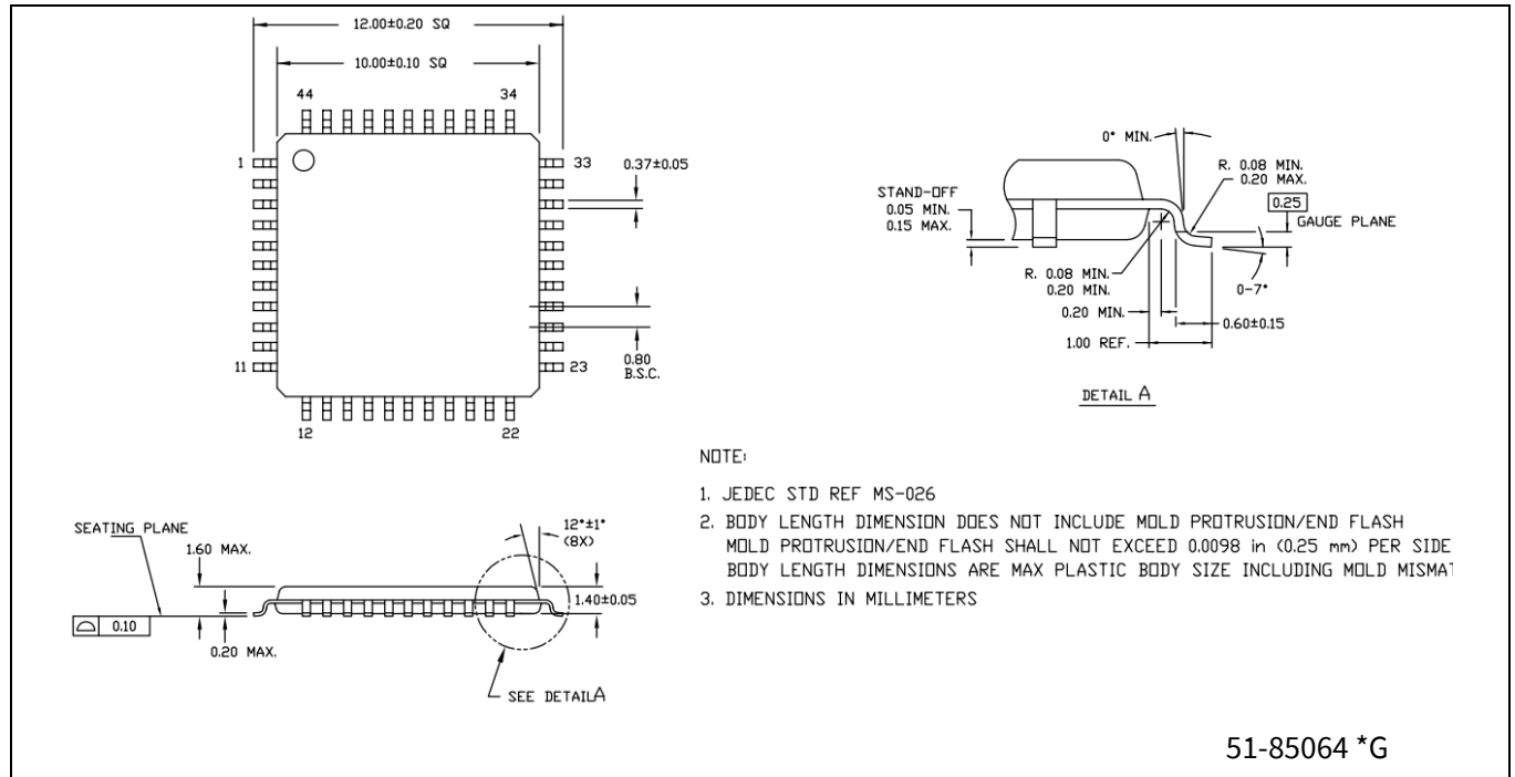
Figure 6 44LD TQFP (10 × 10 × 1.4 mm) A44S (PG-TQFP-44) package outline
