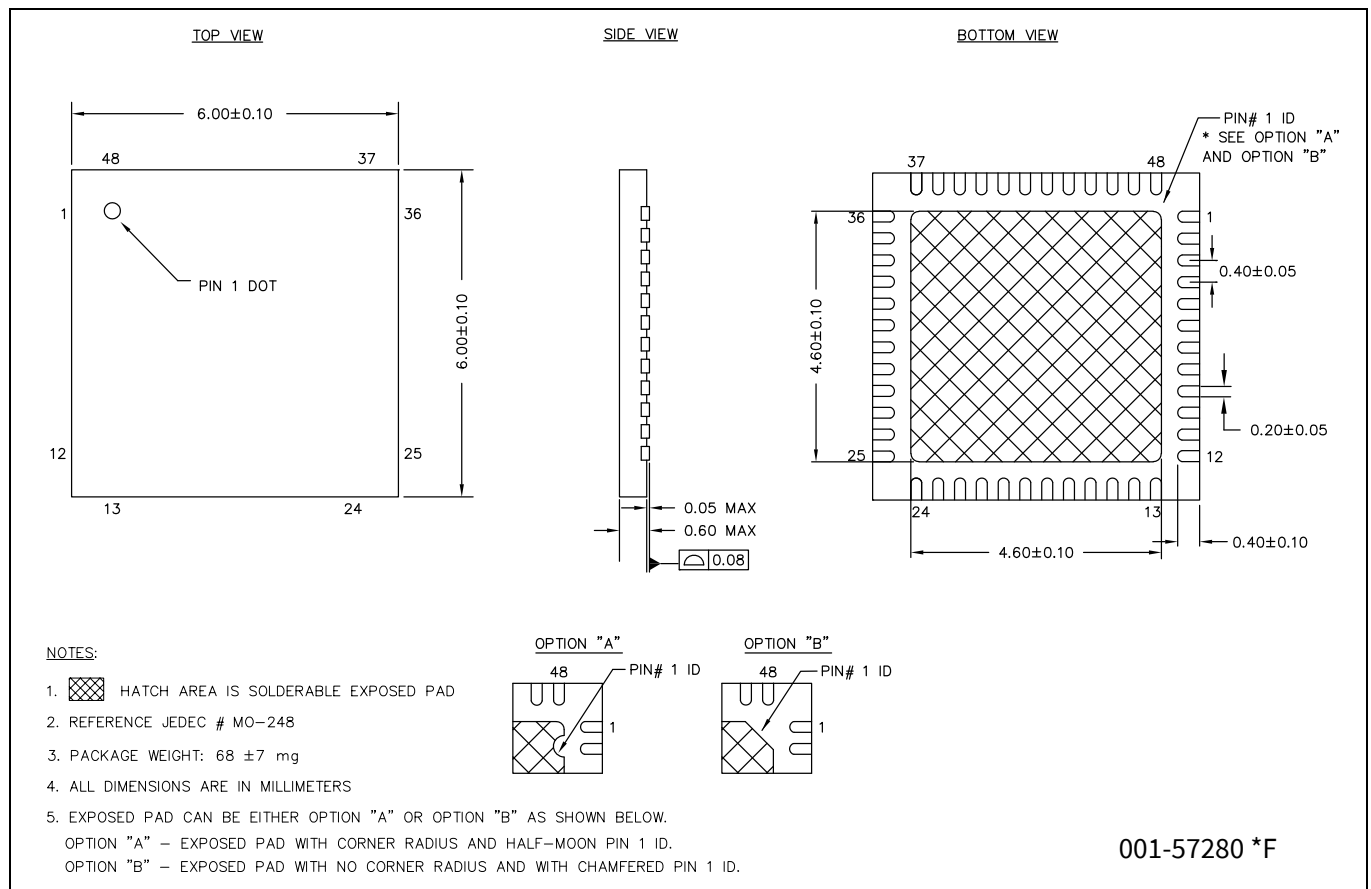
Figure 8 48L QFN (6 × 6 × 0.6 mm) LR48A/LQ48A (4.6 × 4.6 E-PAD) SAWN (PG-VQFN-48) package outline
