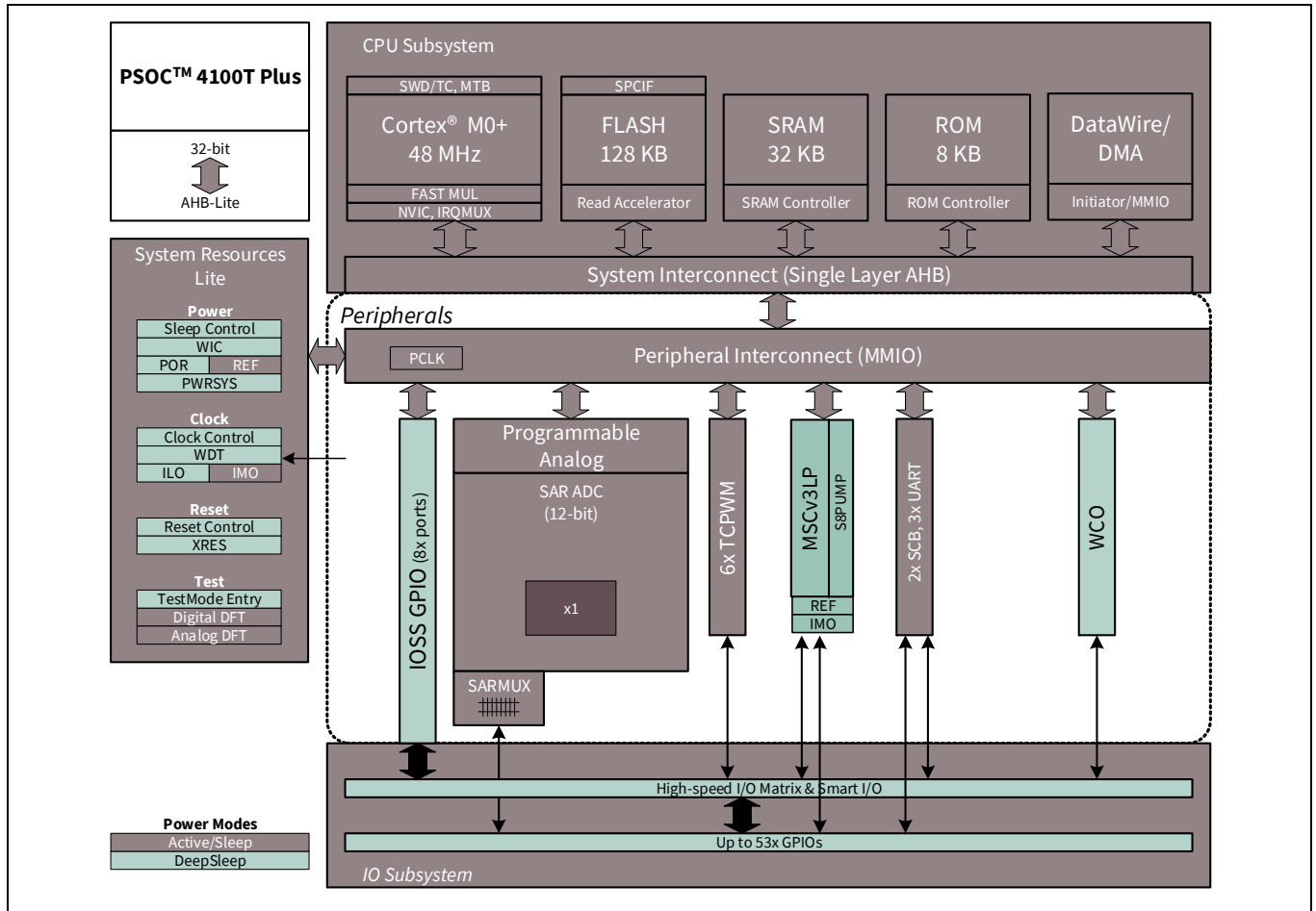
Figure 2 Block diagram
