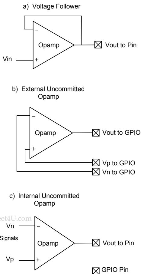
Figure 8-6. Opamp Configurations
