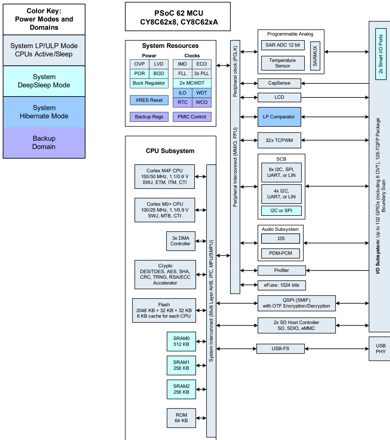
Figure 2. Block Diagram
