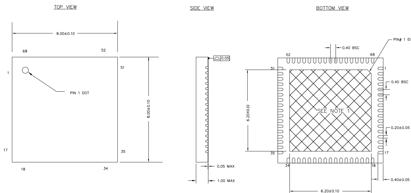
Figure 24. 68 QFN 8 × 8 × 1 mm
