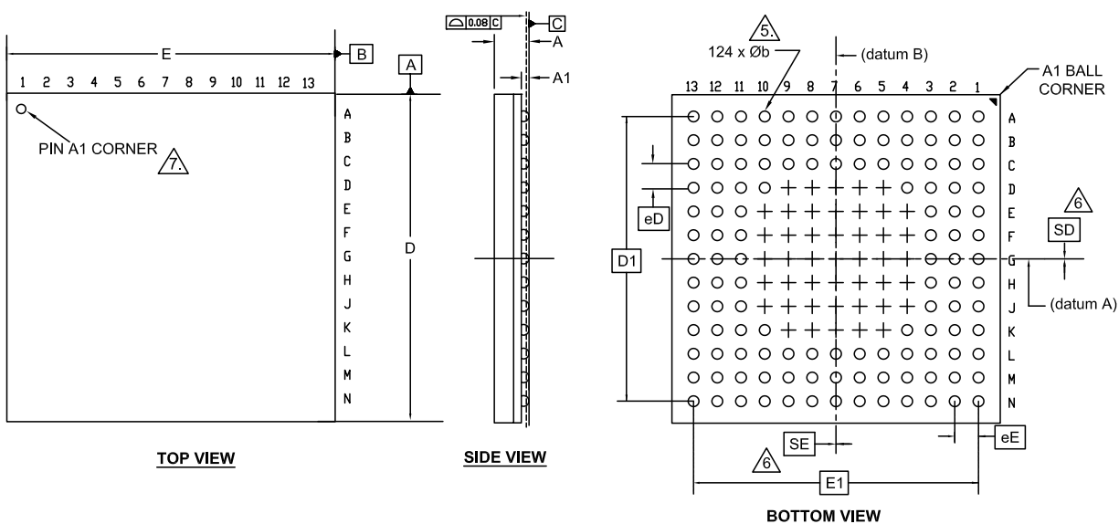
Figure 23. 124-BGA 9.0 × 9.0 × 1.0 mm
