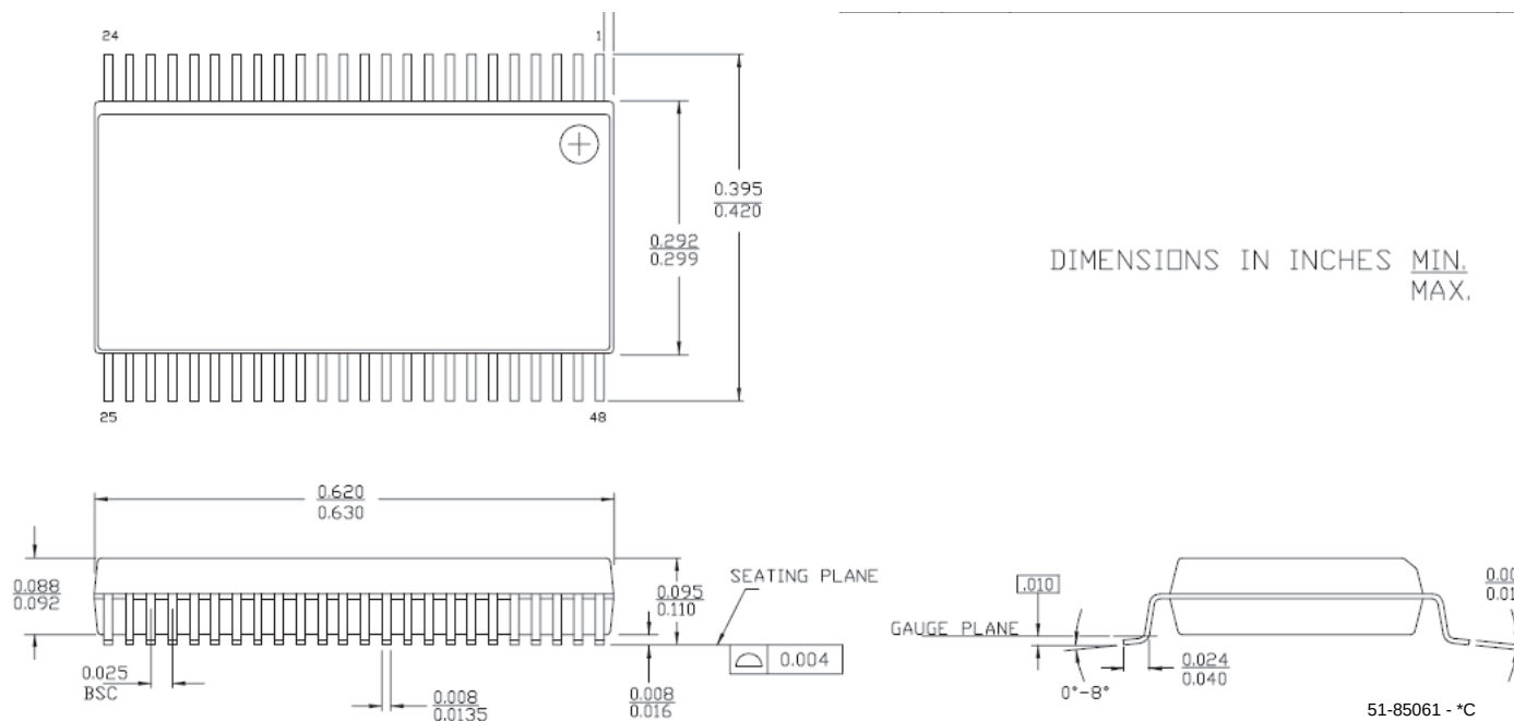
Figure 5-2. 48-Lead (300-Mil) SSOP
