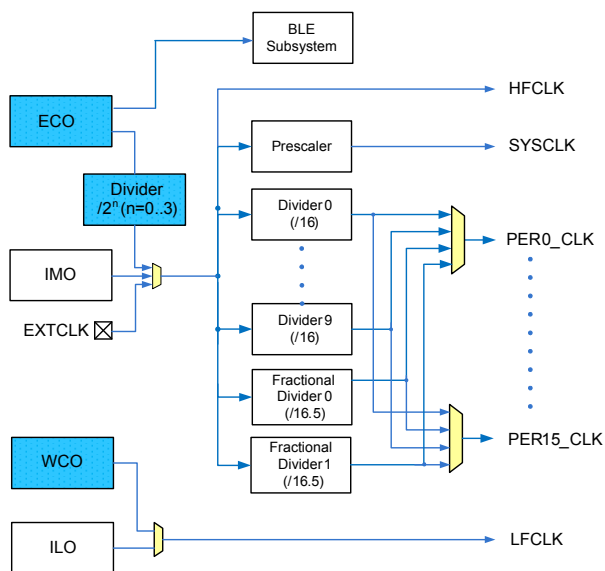
Figure 2. Clock Control
