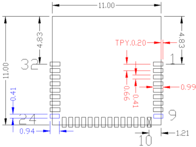
Figure 4. Host Layout Pattern for CYBLE-214009-00
