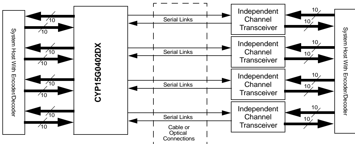
Figure 1. CYP15G0402DX HOTLink II™ System Connections
