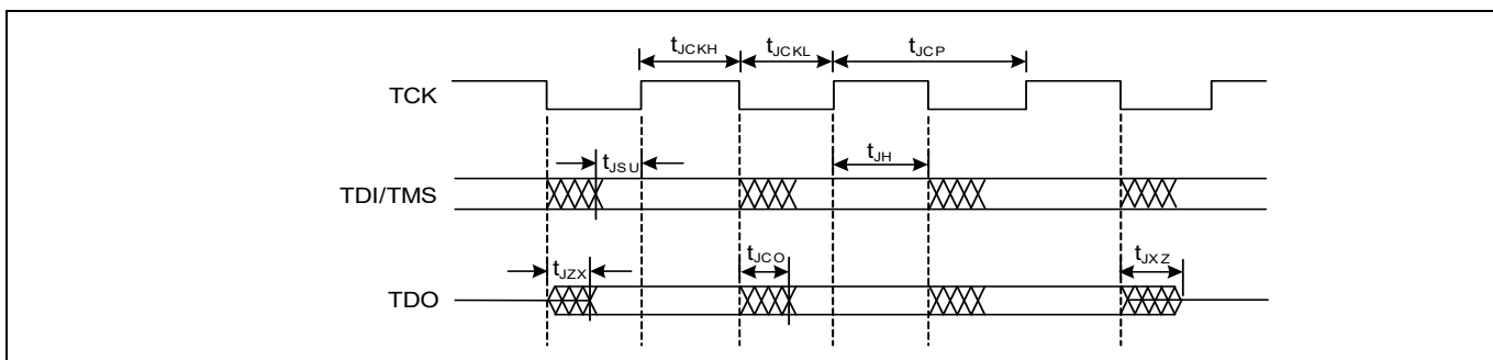
Figure 27-21 JTAG specifications
