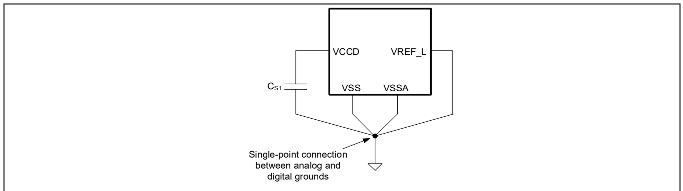
Figure 27-2 Smoothing capacitor
