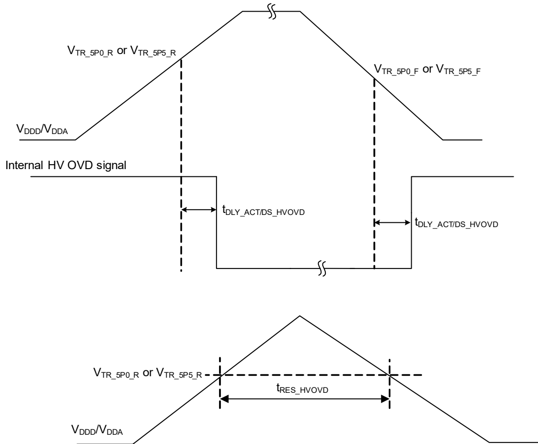
Figure 26-17.High-Voltage OVD Specifications
