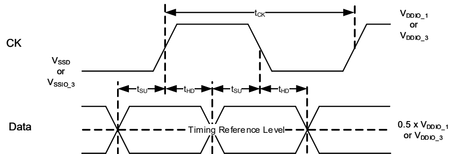
Figure 26-30.DDR Write Timing Reference Level
