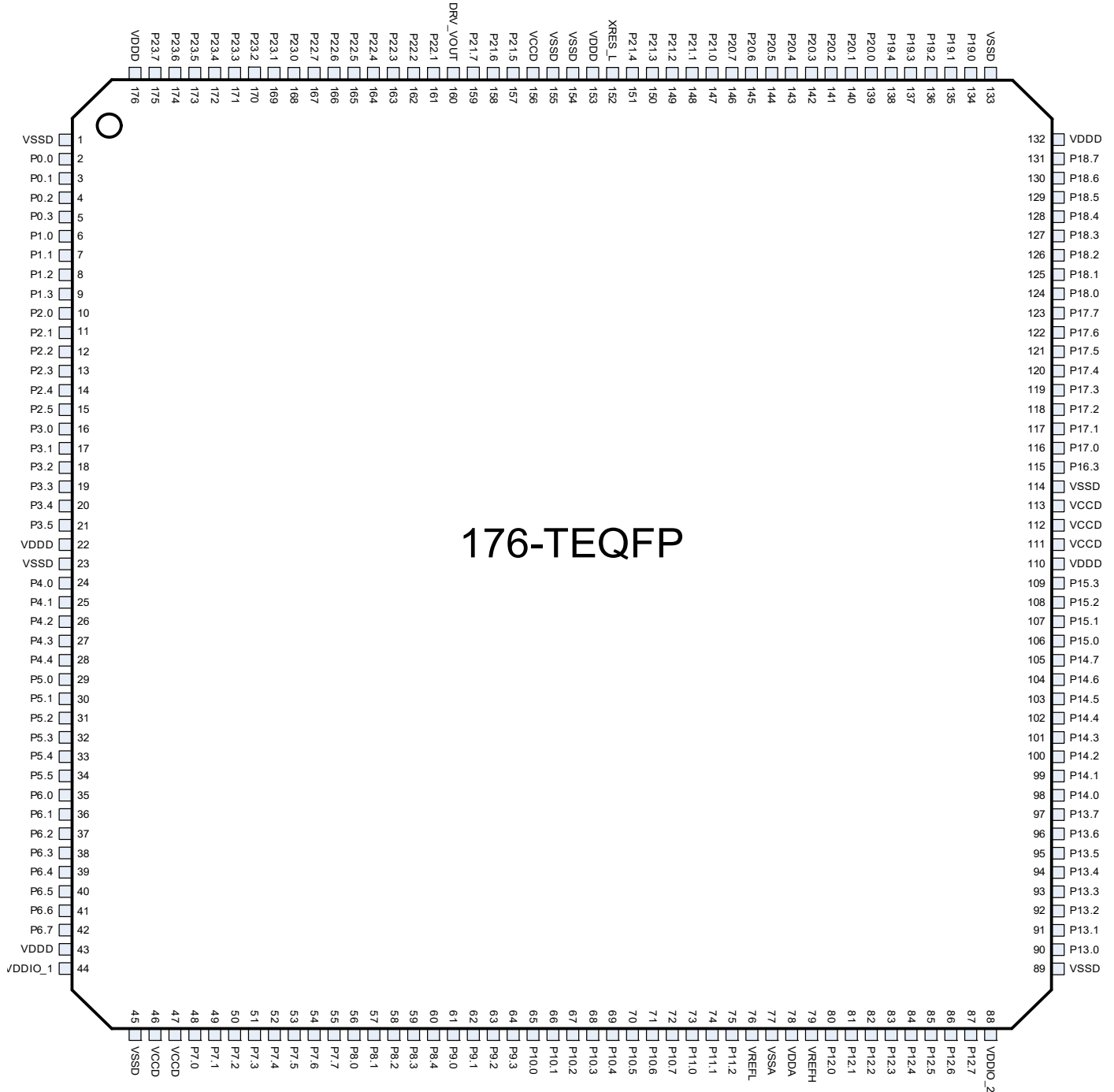
Figure 9-5.176-TEQFP Pin Assignment
