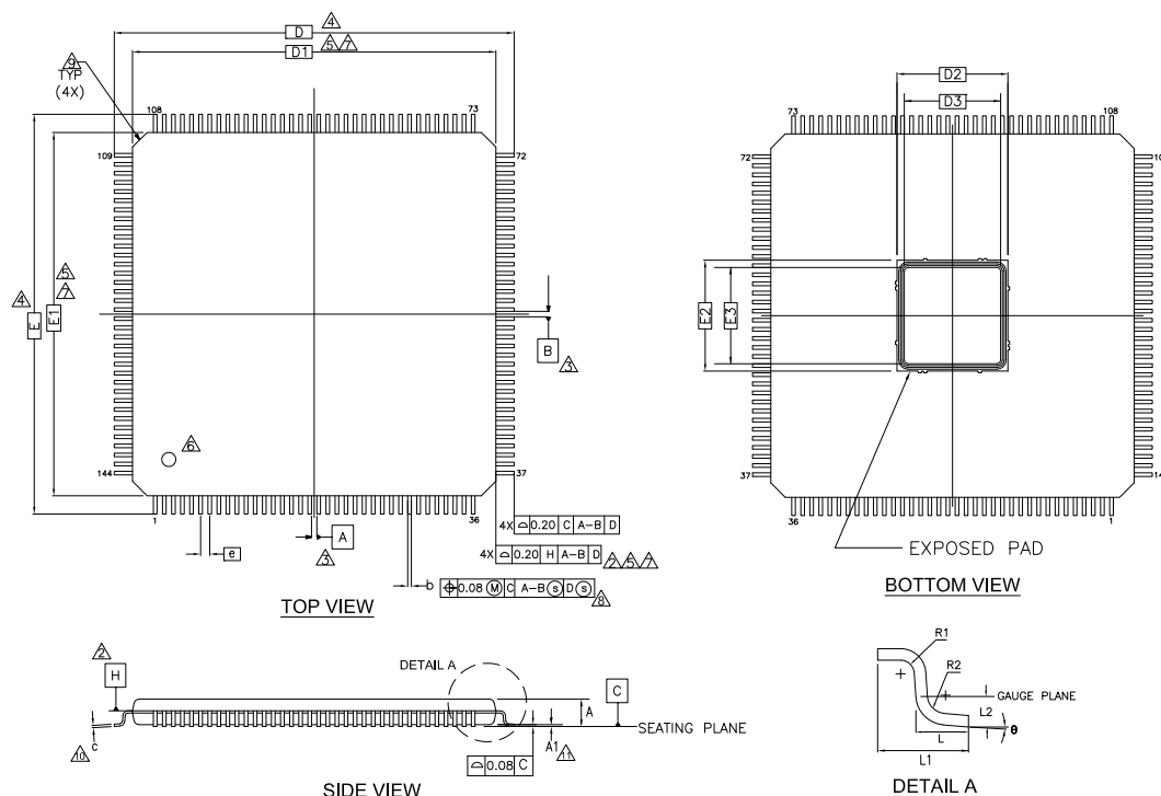
Figure 28-2.Package Outline – 144-TEQFP
