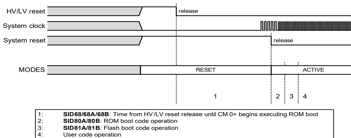
Figure 26-3.Reset Sequence
