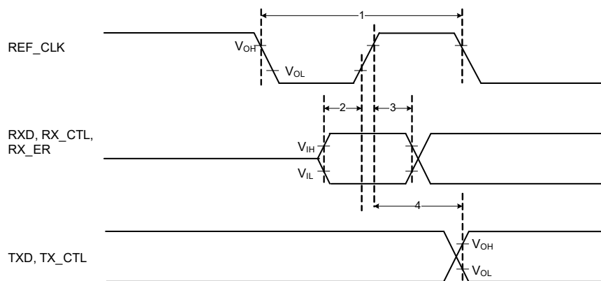
Figure 26-27.RMII Timing Diagram
