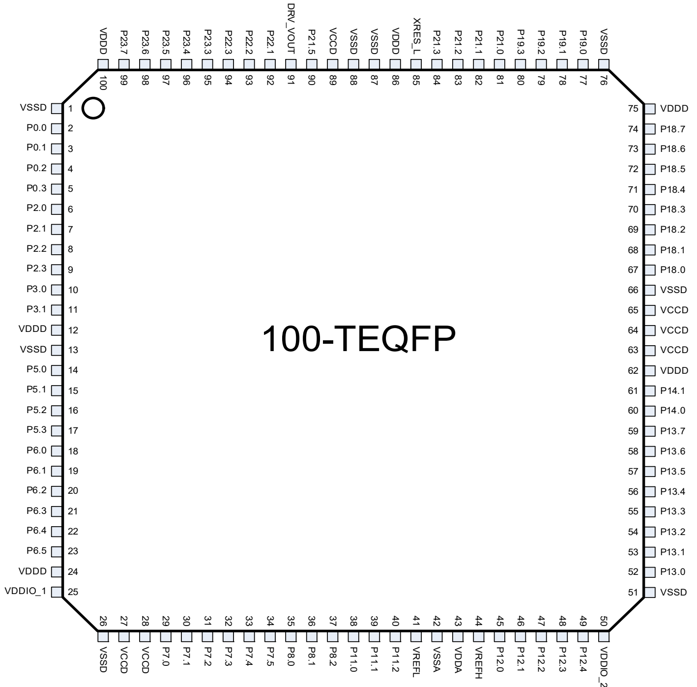
Figure 9-1.100-TEQFP Pin Assignment
