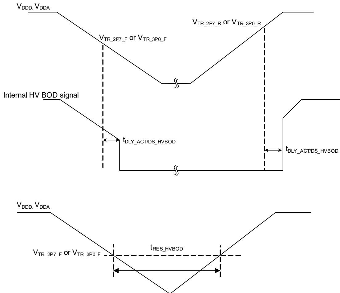
Figure 26-15.High-Voltage BOD Specifications
