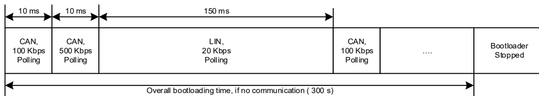
Figure 29-1.Bootloading Sequence
