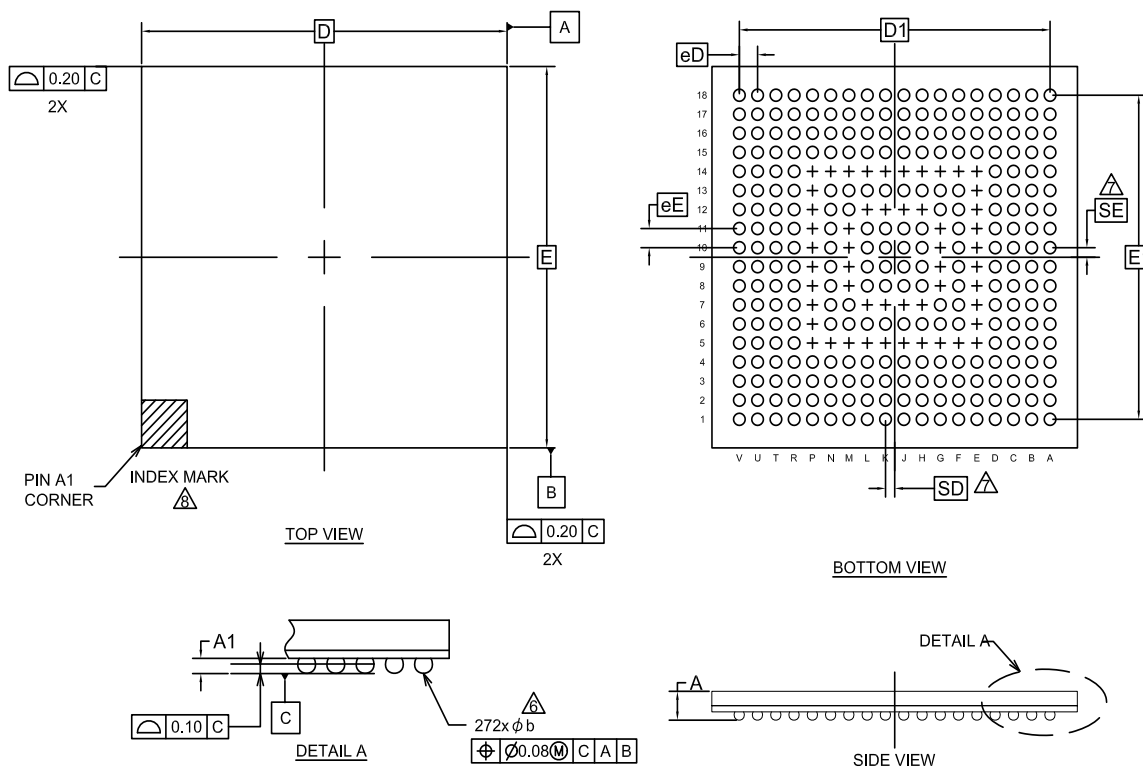
Figure 28-4.Package Outline – 272-BGA
