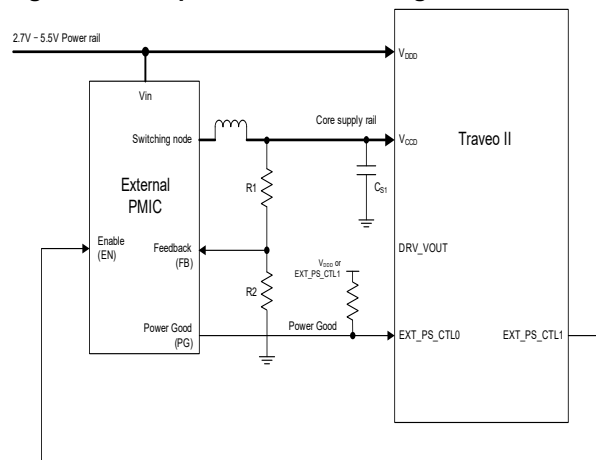
Figure 3-2. Sample Core External Regulator with PMIC/LDO
