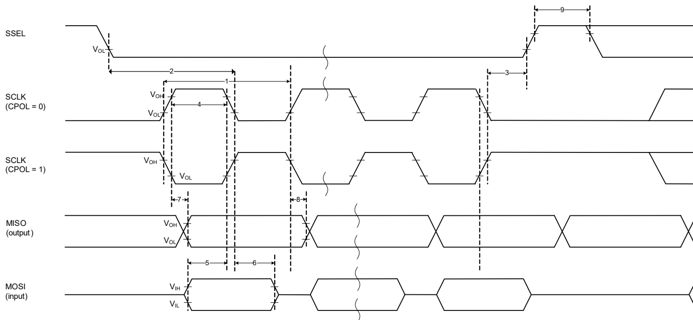
Figure 26-12. SPI Slave Timing Diagrams with HIGH Clock Phase
