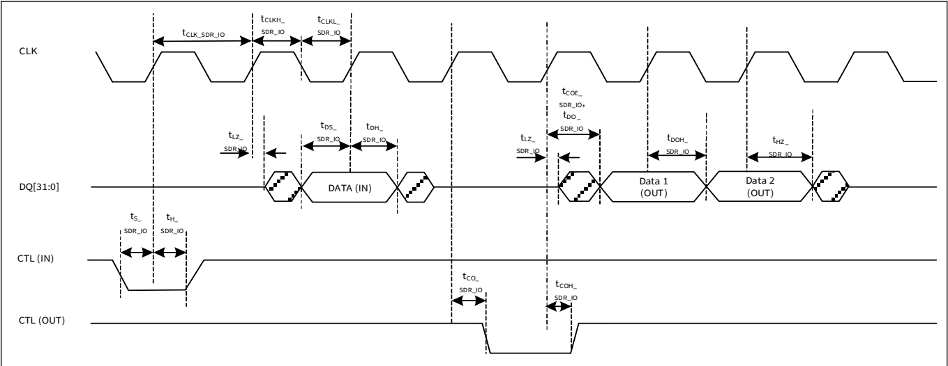
Figure 15 GPIF III timing in LVCMOS SDR IO synchronous mode (see Table 45 )
