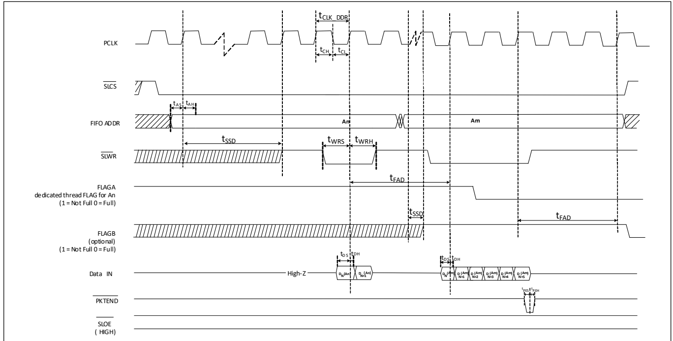
Figure 21 Synchronous DDR slave FIFO write cycle timing diagram
