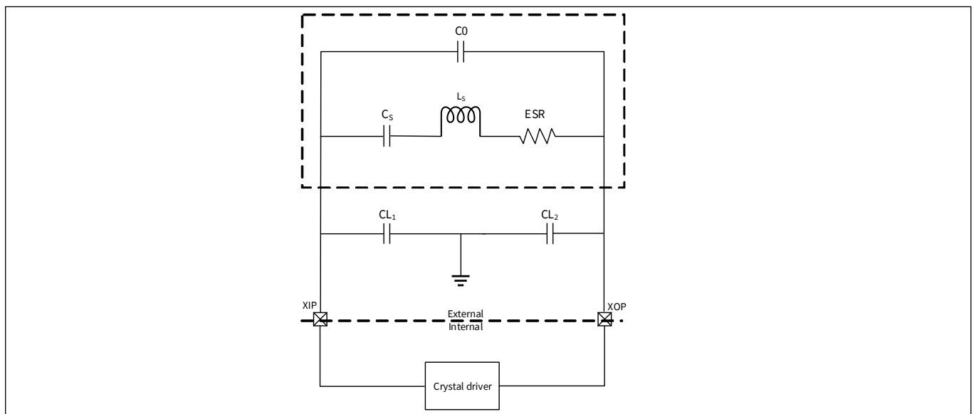
Figure 3 Oscillator circuits
