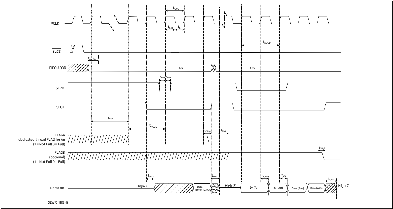
Figure 17 Synchronous SDR slave FIFO read cycle timing
