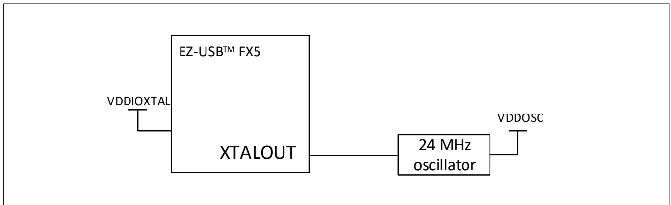
Figure 4 External clock input
