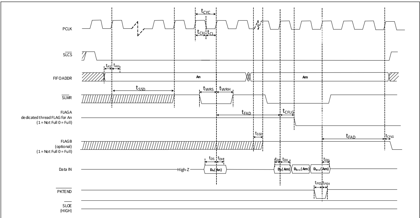
Figure 19 Synchronous SDR slave FIFO write cycle timing
