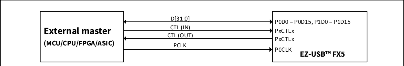
Figure 14 LVCMOS SDR IO GPIF III interface example
