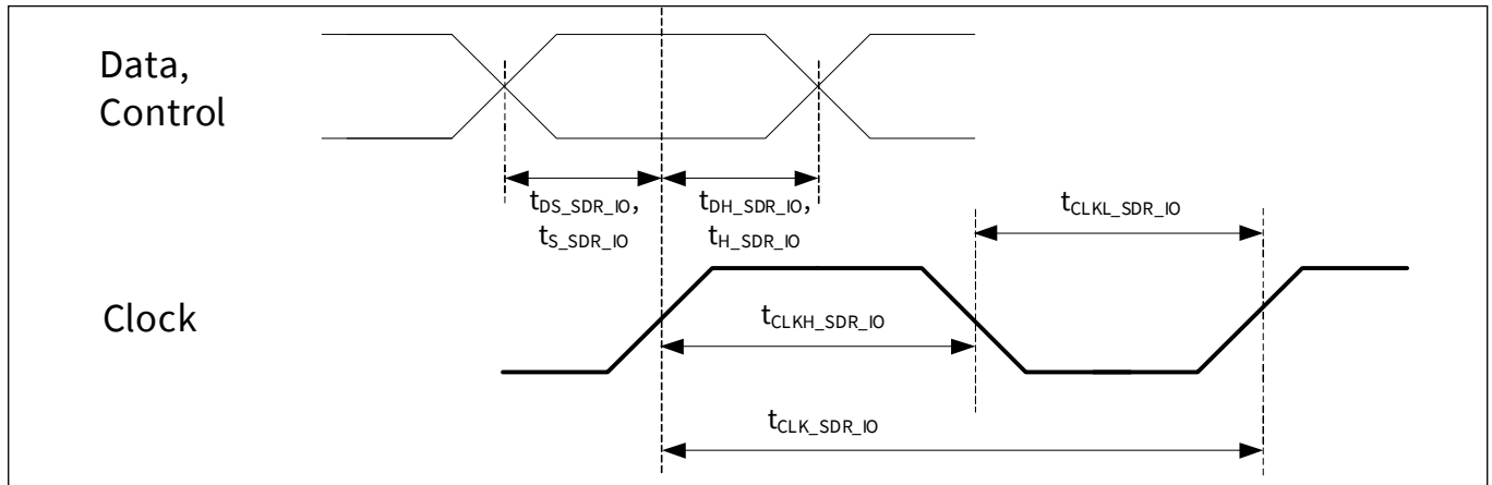
Figure 13 LVC MOS SDR IO clock and data timing
