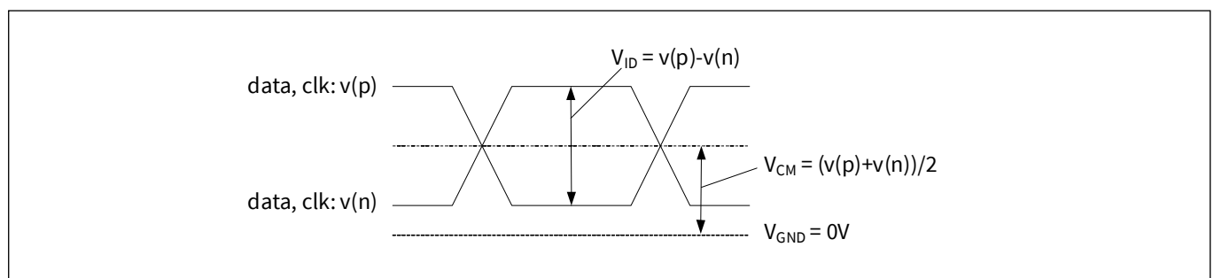
Figure 8 LVDS VCM and VID illustration
