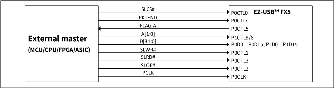
Figure 18 Slave FIFO write interface example
