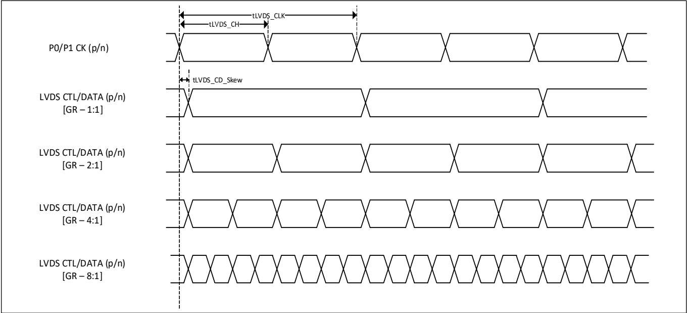
Figure 22 LVDS write cycle timing diagram (for the timing parameters, see Table 41 )
