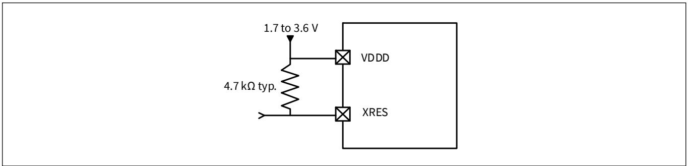
Figure 5 XRES connection diagram
