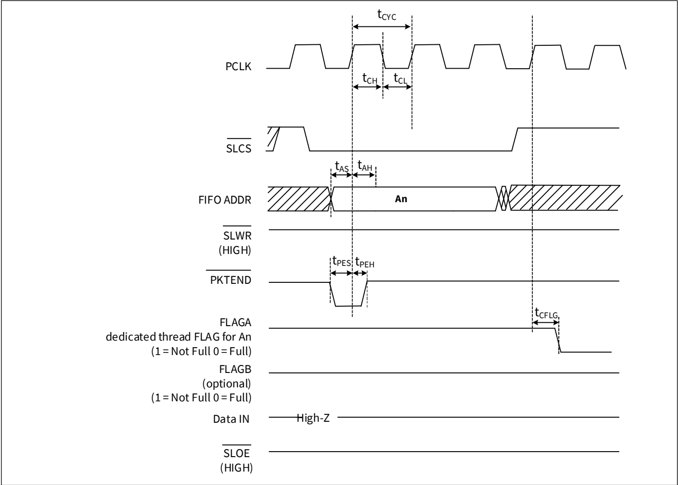
Figure 20 Synchronous SDR slave FIFO ZLP write cycle timing
