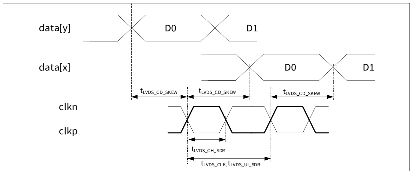
Figure 9 LVDS SDR clock and data timing
