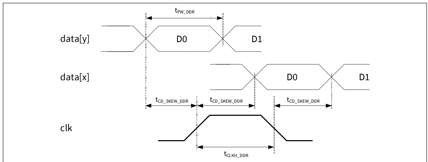
Figure 12 LVC MOS DDR clock and data timing
