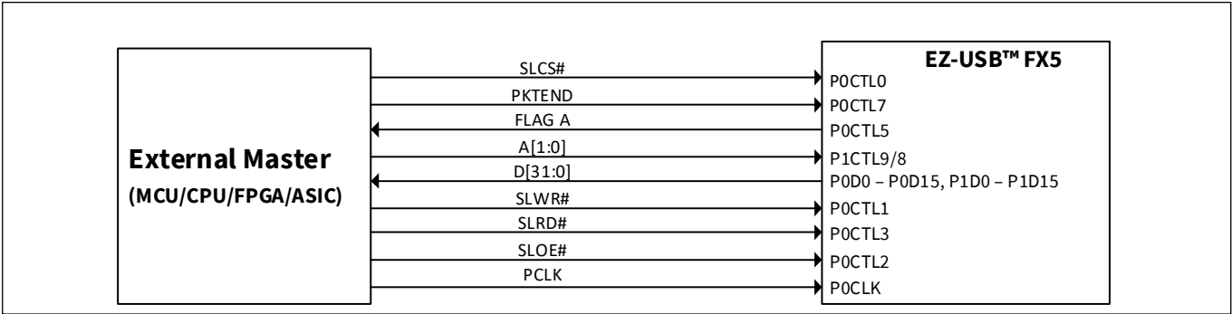
Figure 16 Slave FIFO read interface example
