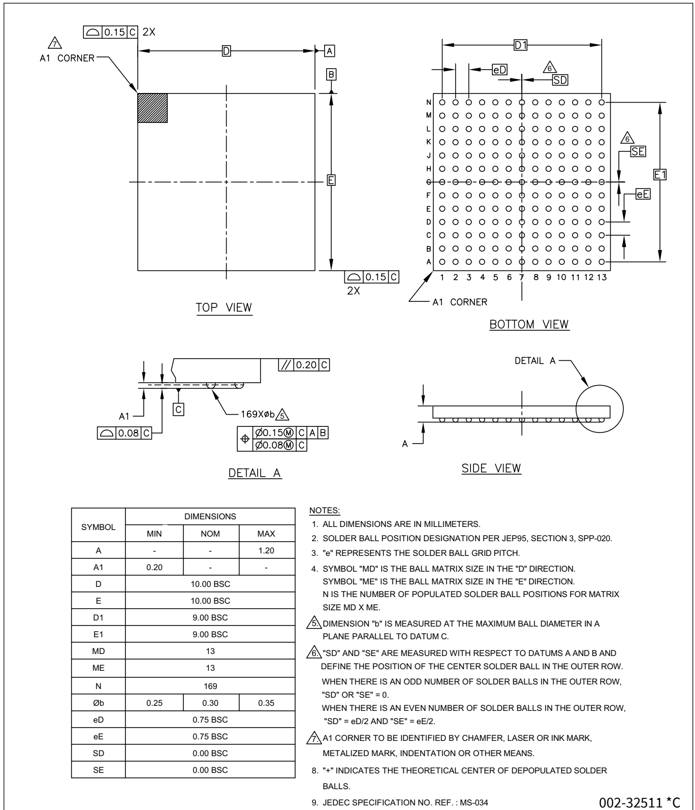
Figure 23 169-ball FBGA (10 × 10 × 1.2 mm) FCA169 package outline, 002-32511
