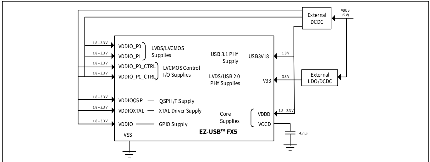
Figure 7 Power system requirement block diagram
