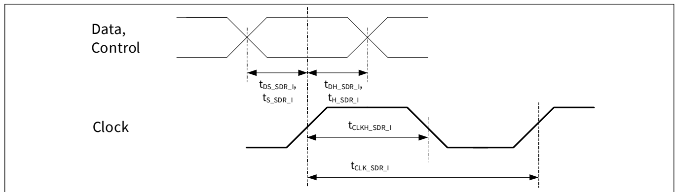
Figure 11 LVC MOS SDR input only clock and data timing
