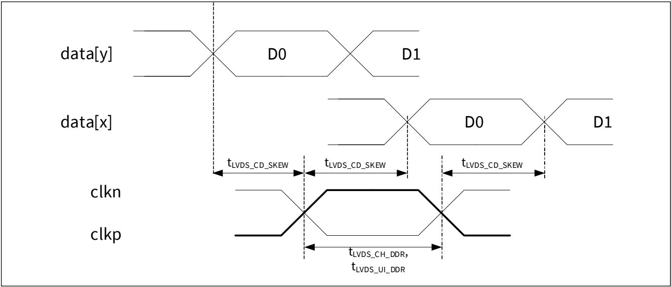
Figure 10 LVDS DDR clock and data timing
