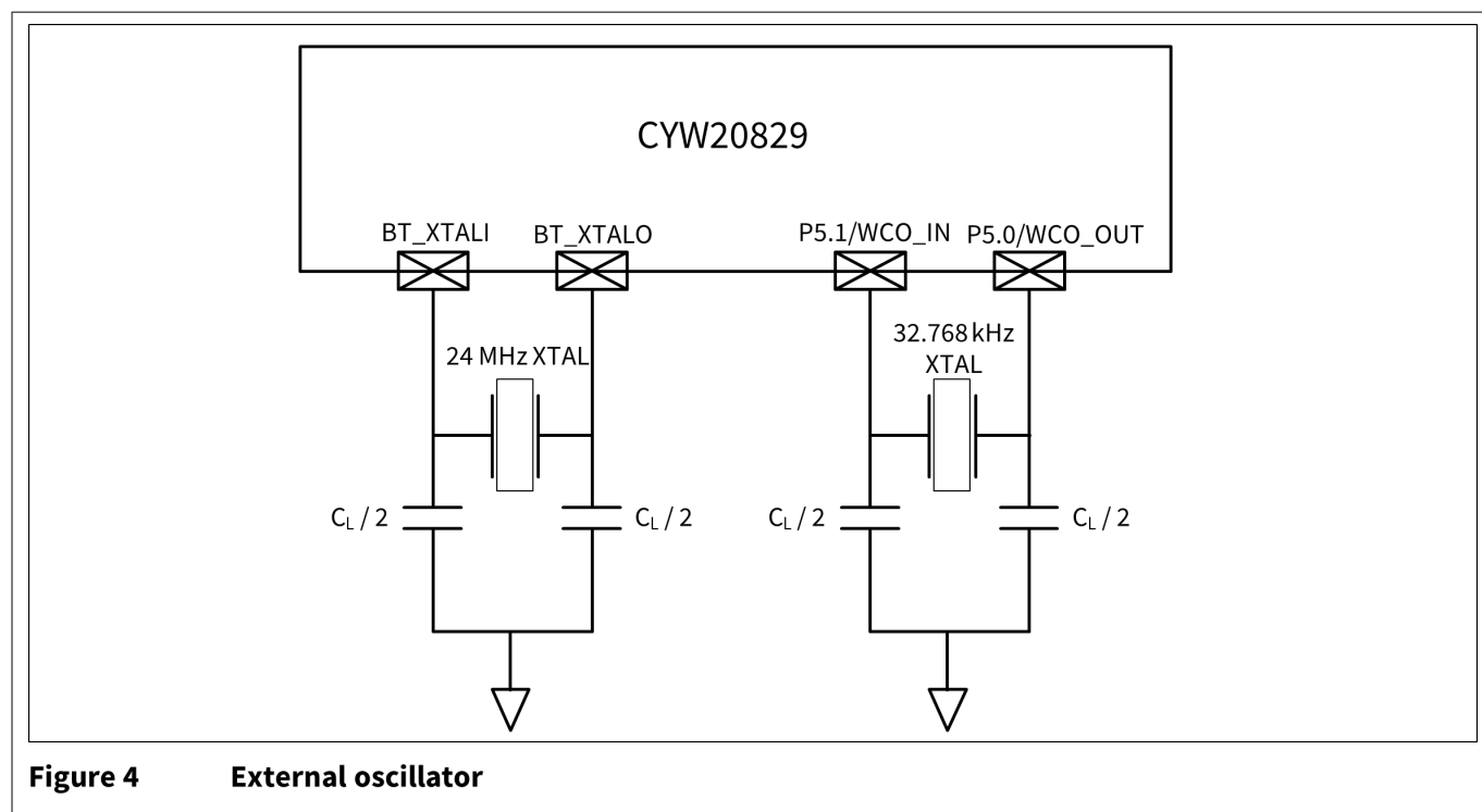
Figure 4 External oscillator
