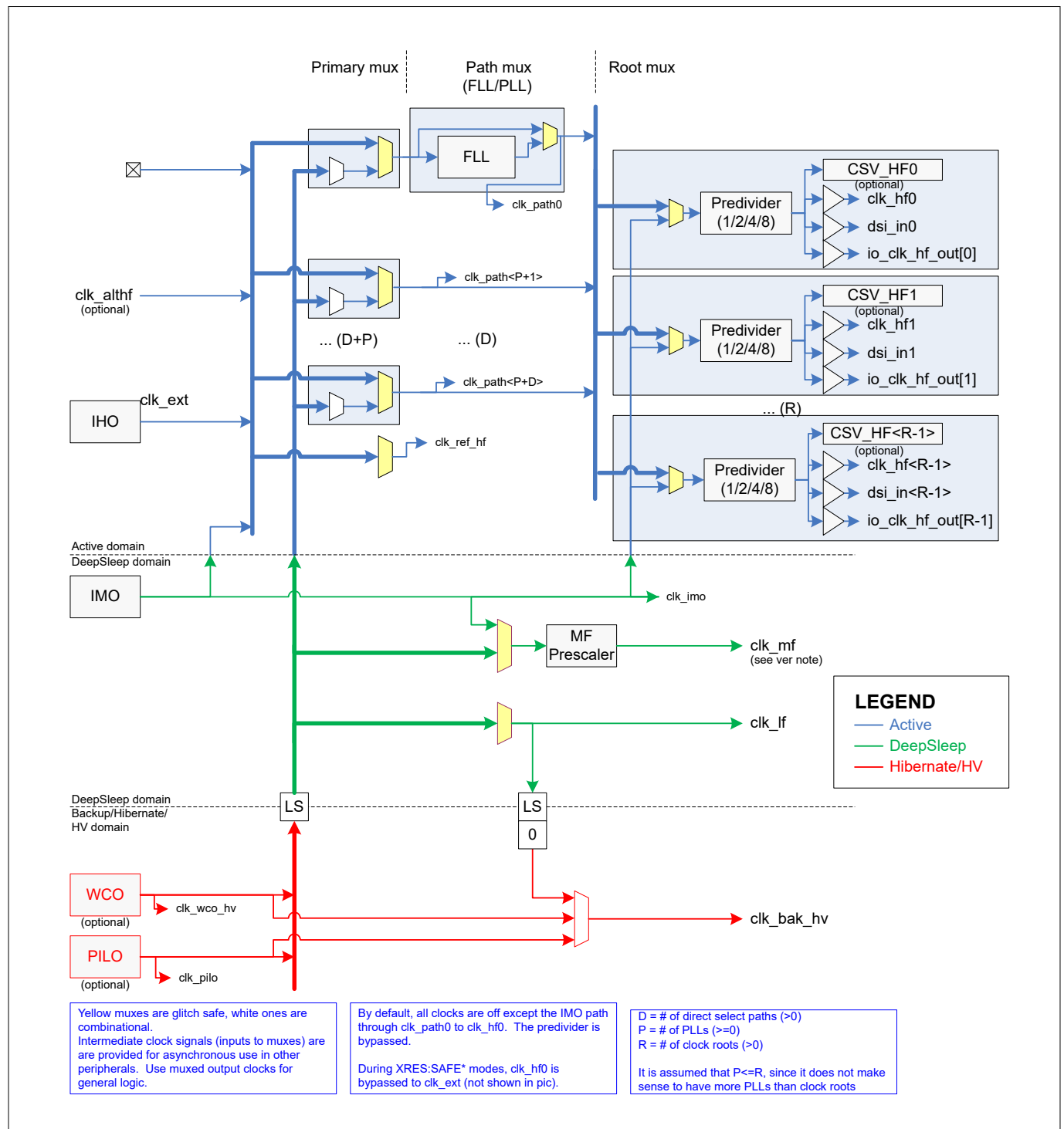
Figure 3 CYW20829 clocking diagram with corresponding oscillators
