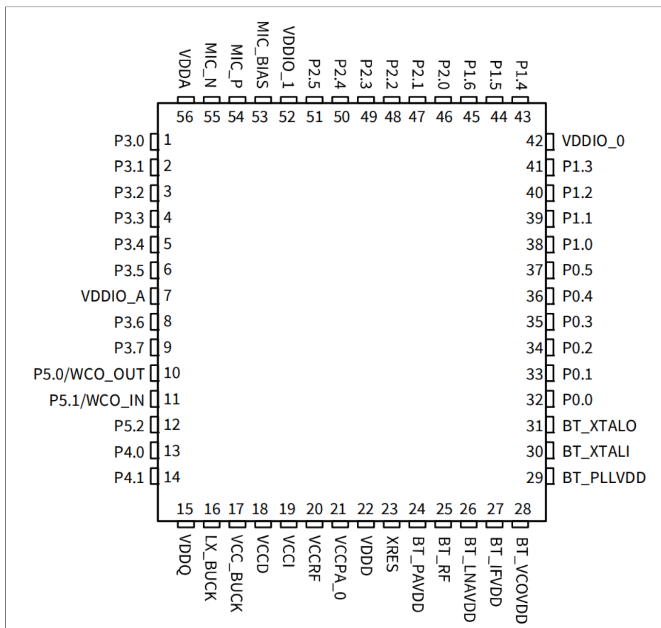
Figure 6 Device pinout for 56-lead package
