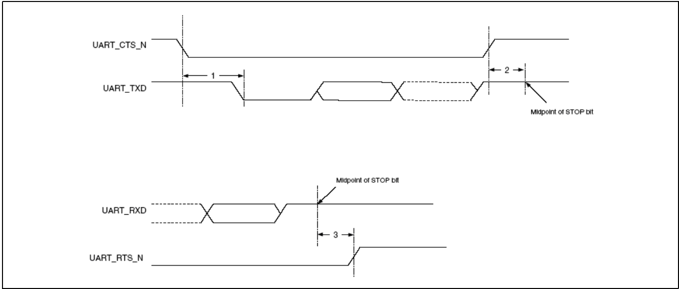
Figure 8 UART timing
