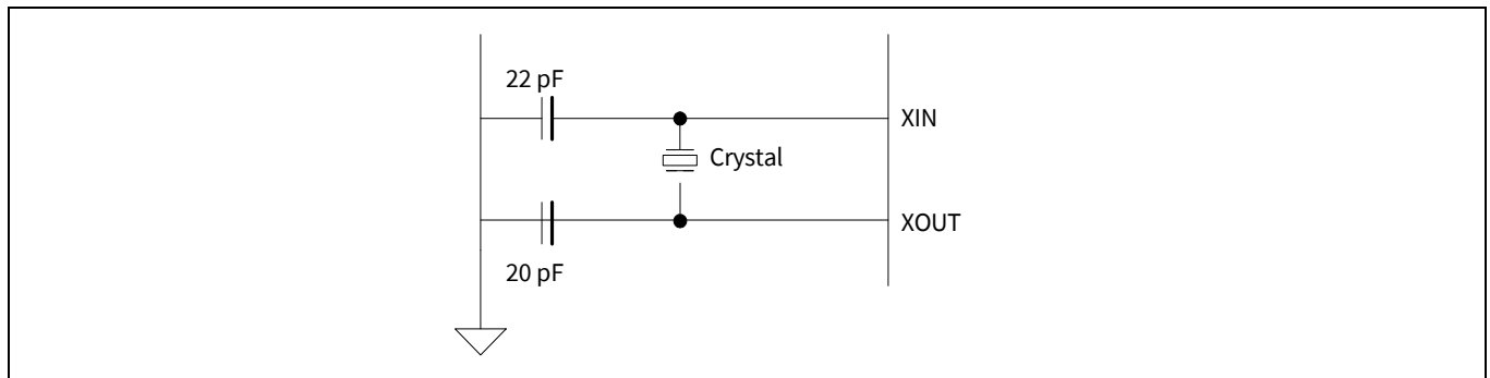
Figure 3 Recommended oscillator configuration — 12 pF load crystal
