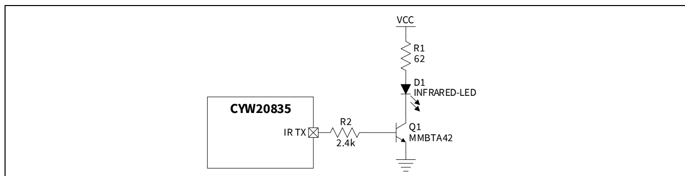
Figure 6 Infrared TX
