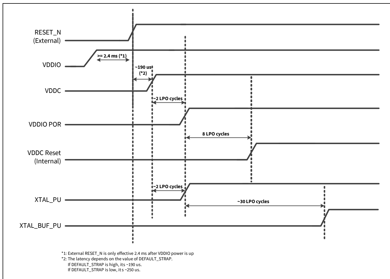
Figure 1 Power-on reset (POR) timing
