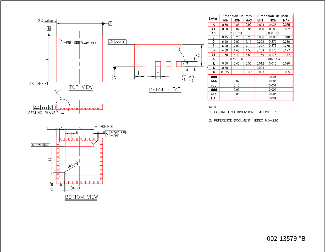
Figure 14 60-lead QFN (7 × 7 × 0.90 mm) LT60A (PG-VQFN-60), package outline
