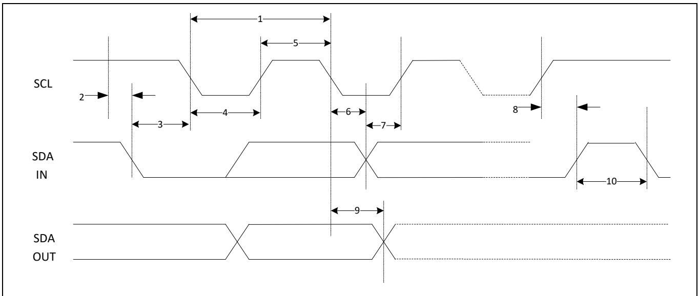
Figure 11 I 2 C interface timing diagram
