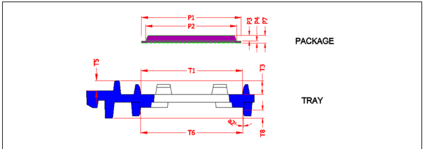
Figure 15 QFN package and tray dimensions
