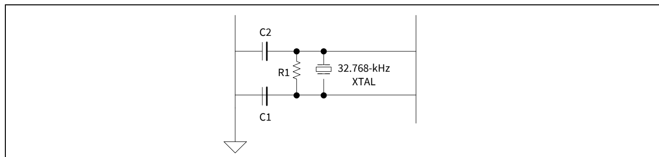
Figure 4 32-kHz oscillator block diagram
