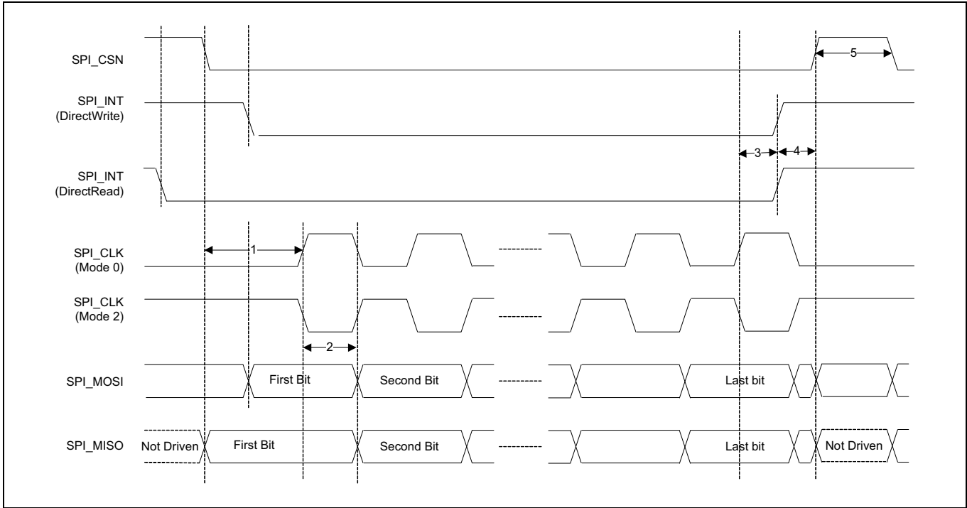
Figure 9 SPI timing, mode 0 and 2
