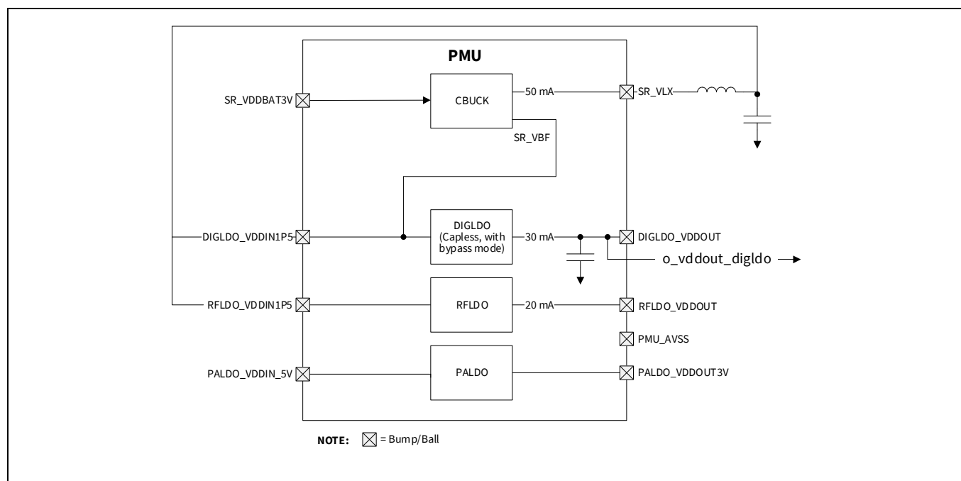
Figure 2 Power management unit
