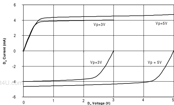
Charge Pump Current vs D_o Voltage I_{cp}=High
