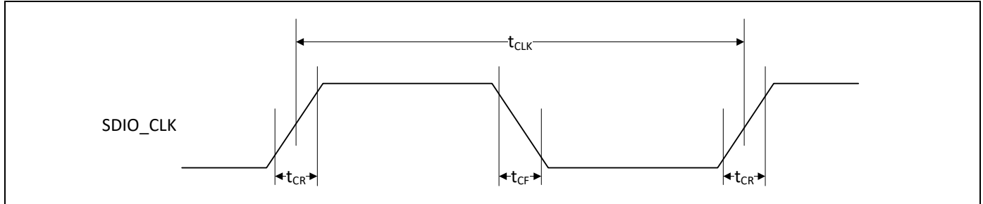
Figure 34. SDIO Clock Timing (SDR Modes)
