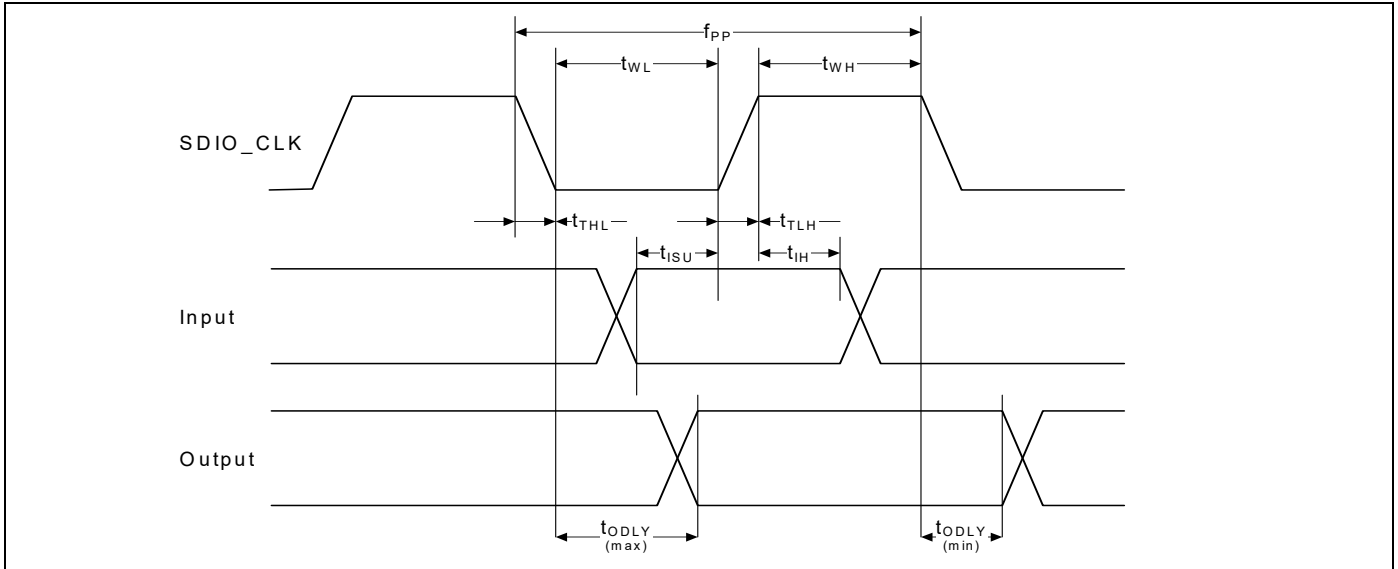
Figure 29. SDIO Bus Timing (Default Mode)
