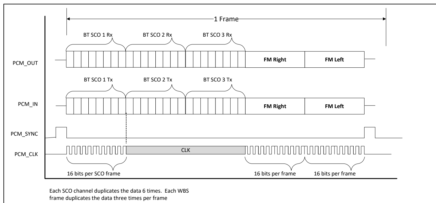
Figure 9. Functional Multiplex Data Diagram
