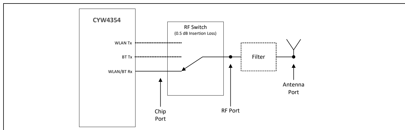
Figure 35. RF Port Location for Bluetooth Testing
