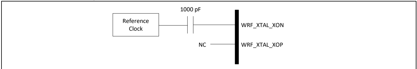
Figure 6. Recommended Circuit to Use With an External Reference Clock
