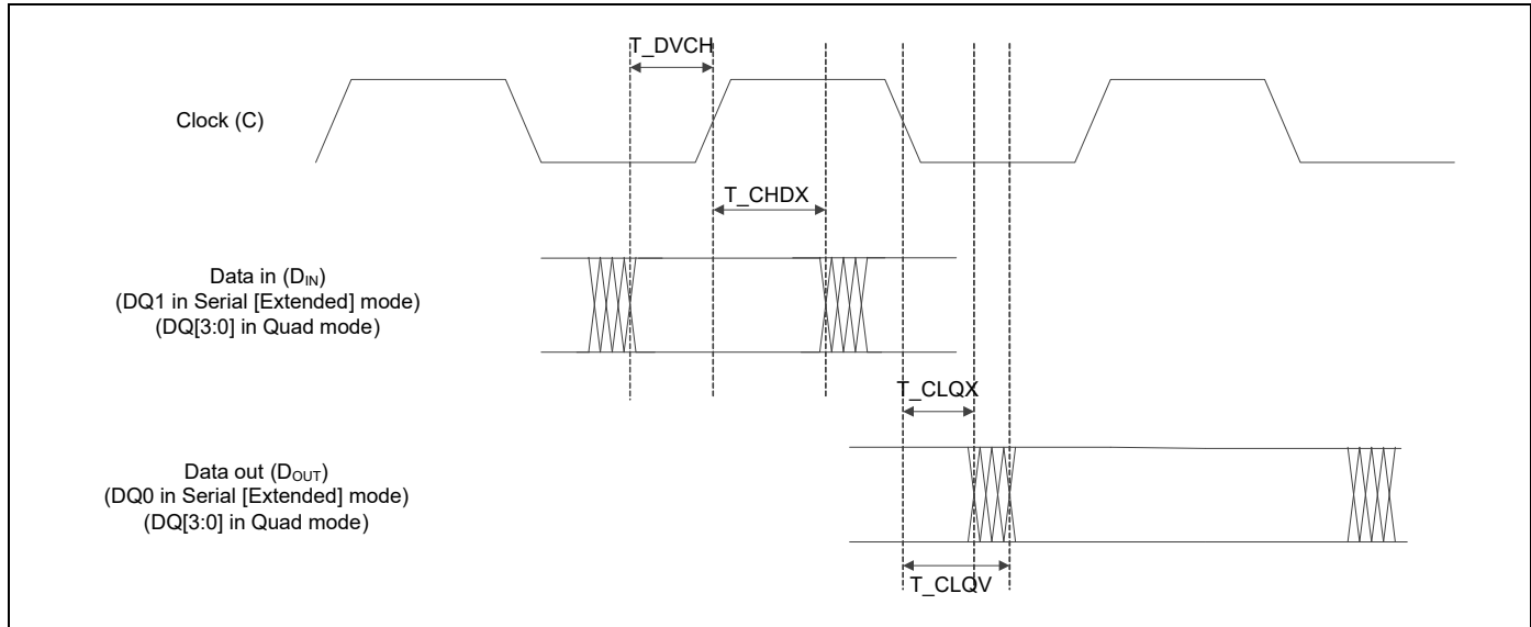
Figure 17. SPI Flash Timing Parameters Diagram
