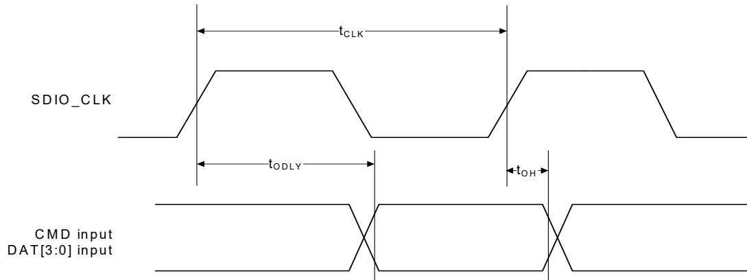
Figure 26. SDIO Bus Output Timing (SDR modes up to 50 MHz)
