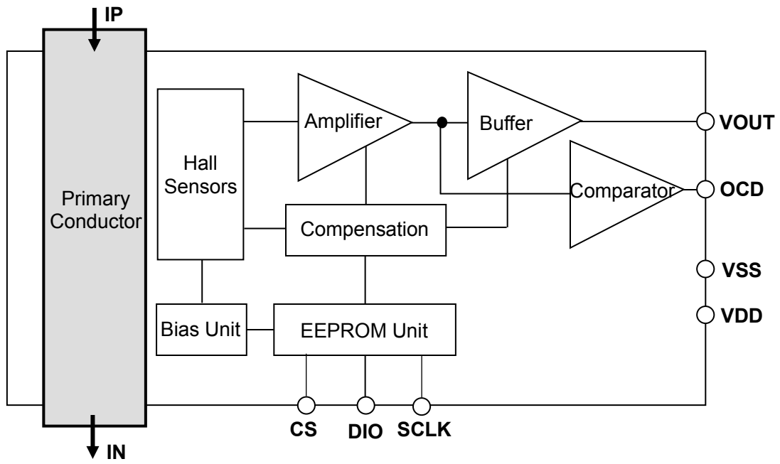
Figure 1. Block diagram of CZ-3815
