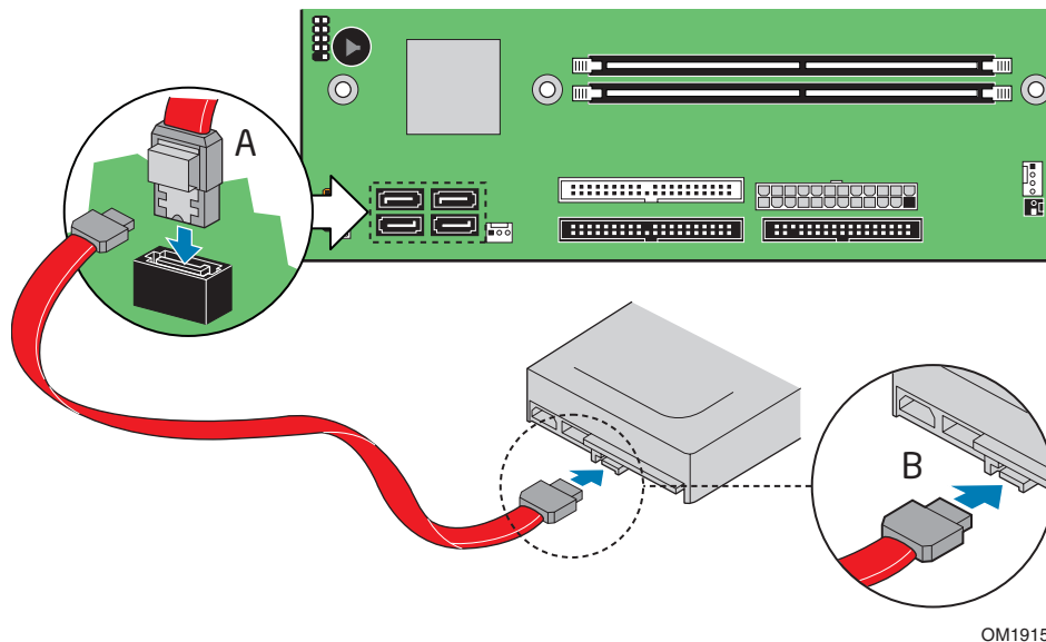
Figure 18. Connecting the Serial ATA Cable
