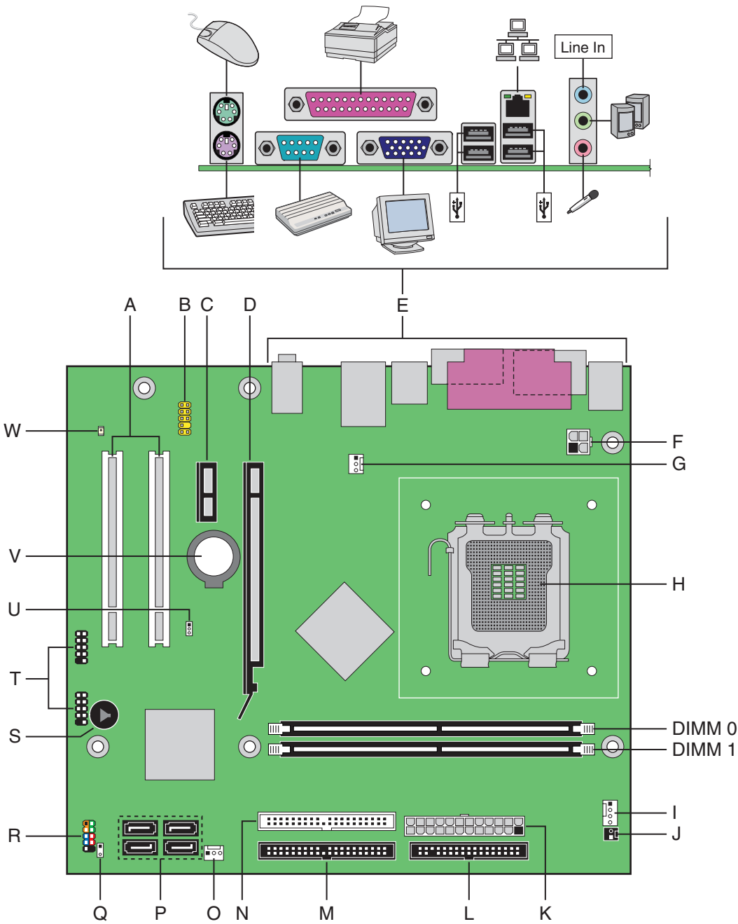
Figure 1. Intel Desktop Board D102GGC2 Components
