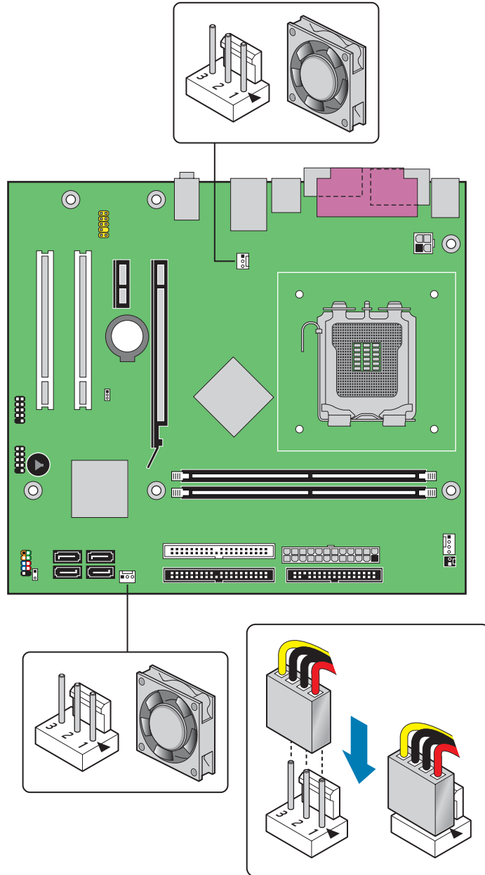
Figure 21. Location of the Chassis Fan Headers
