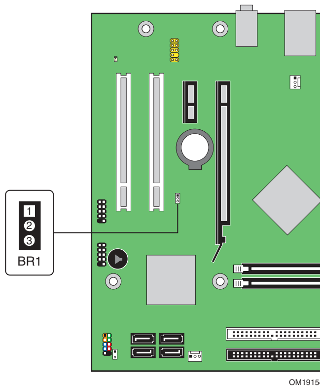
Figure 24. Location of the BIOS Configuration Jumper Block
