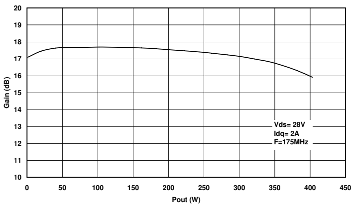
Figure 3. Gain Vs Output Power
