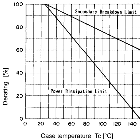
ASO Derating
