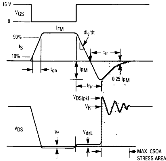
Figure 11. Commutating Waveforms
