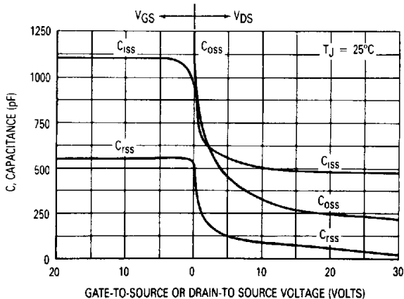
Figure 14. Capacitance Variation
