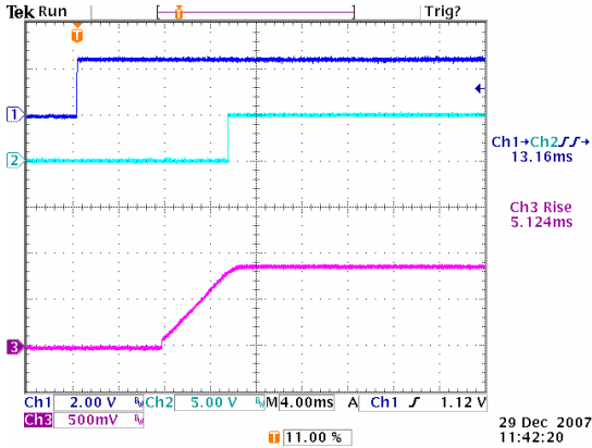
Figure 13: Turn on delay time at 12Vin, 0.9V/40A out (4mS/div) Ch1: Enable, Ch2: PG, Ch3: Vo
