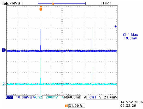
Figure 27: Short Circuit Protection at 12Vin, 1.8V out (40mS/div), Ch1: Vo, Ch2: Io, 50A/div
