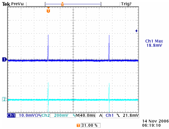
Figure 25: Short Circuit Protection at 12Vin, 0.9V out (40mS/div), Ch1: Vo, Ch2: Io, 50A/div
