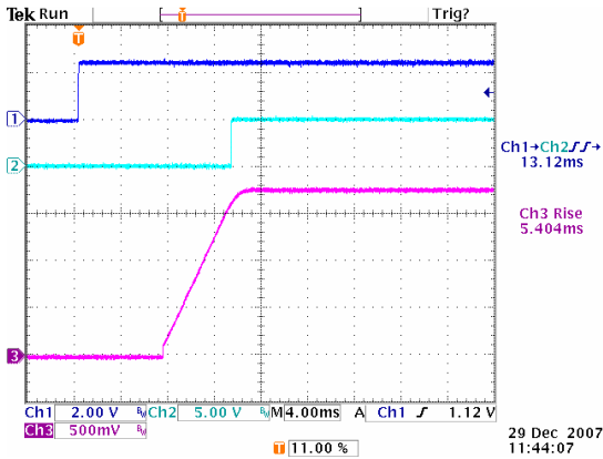
Figure 15: Turn on delay time at 12Vin, 1.8V/40A out (4mS/div) Ch1: Enable, Ch2: PG, Ch3: Vo
