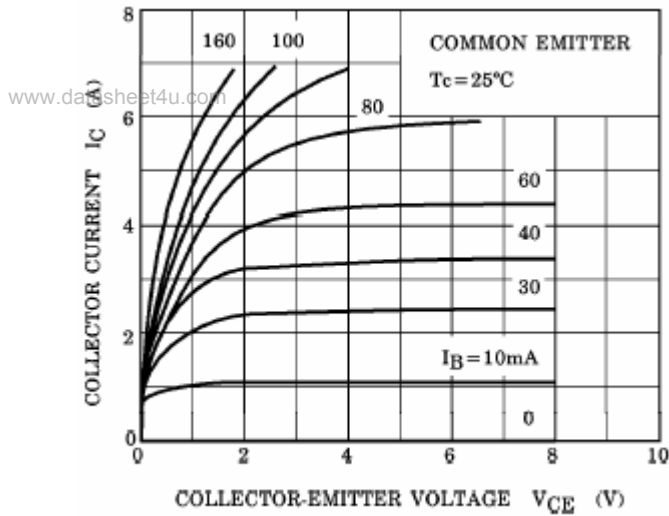
Fig.3 Static Characteristic
