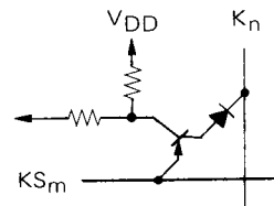
Transistor Switch
