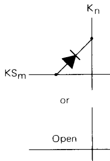
Diode Matrix
