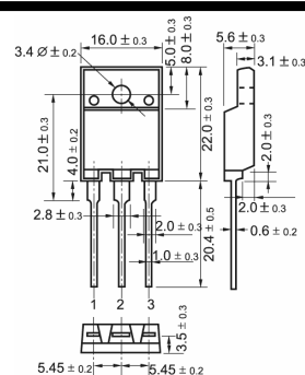
TO-3PML
