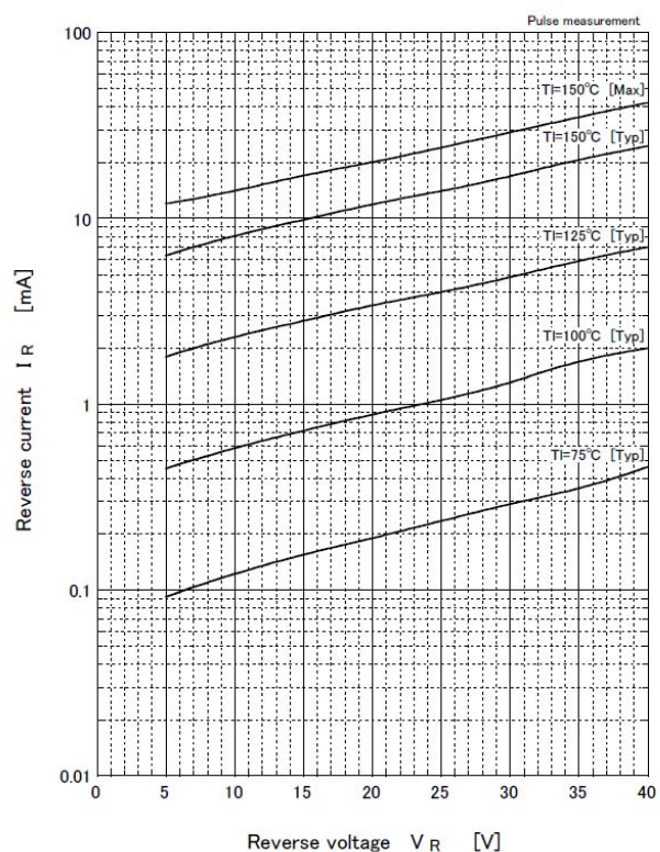
Reverse current
