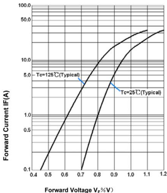
Fig.4 Forward Voltage
