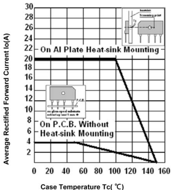
Fig. 1 Derating Curve
