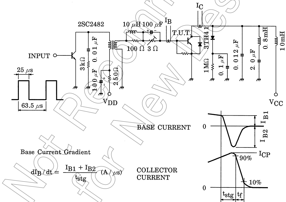
Fig. 1 SWITCHING TIME TEST CIRCUIT
