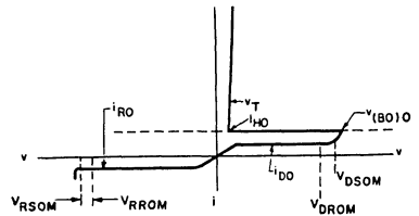
Fig. 2 - Principal voltage-current characteristic for S3705M and S3706E.
