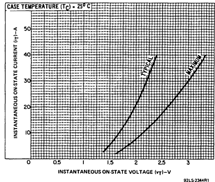
Fig. 5 - Instantaneous on-state current vs. on-state voltage for S3705M and S3706E.
