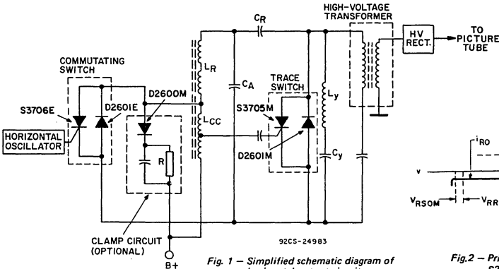
Fig. 1 - Simplified schematic diagram of horizontal output circuit.
