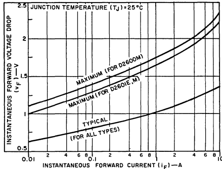
Fig. 10 - Forward-voltage drop vs. forward current for D2600M, D2601E, and D2601M.
