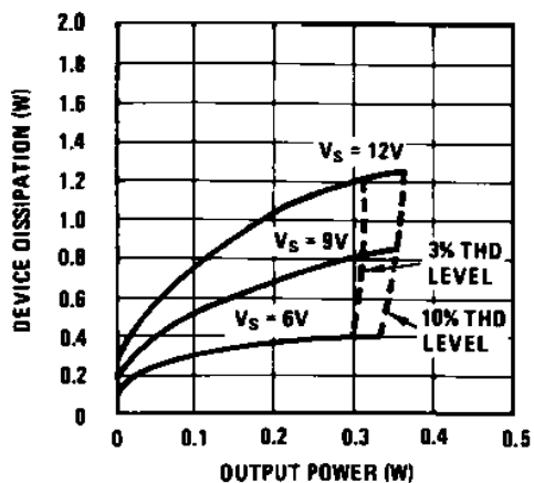
Device Dissipation vs Output Power—4Ω Load
