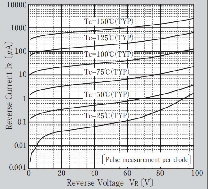
Reverse Current
