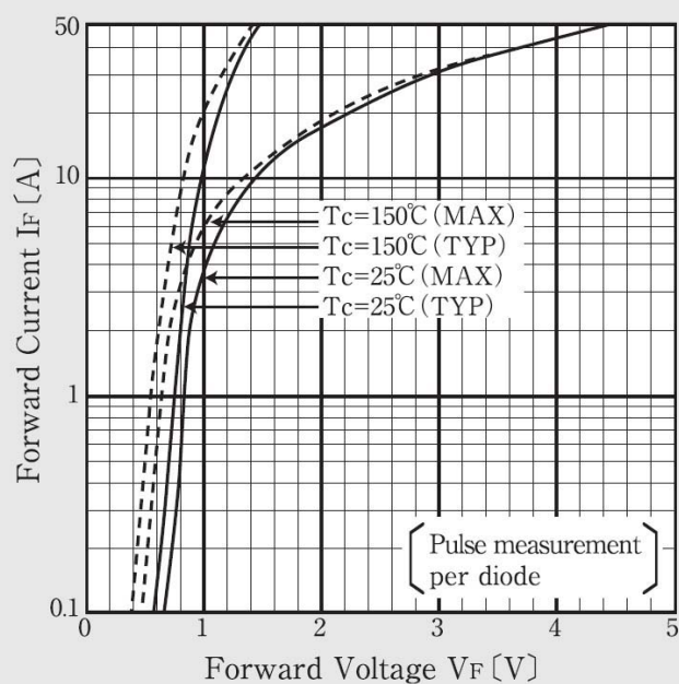
Forward Voltage
