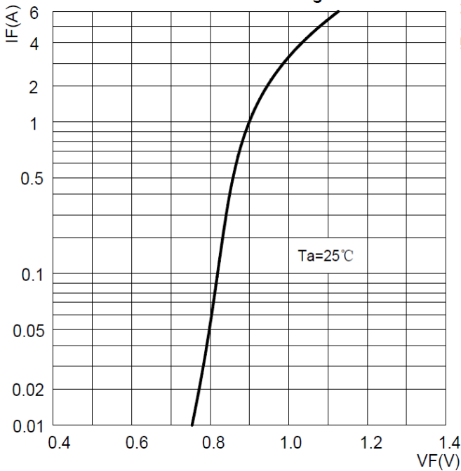
FIG3: Forward Voltage
