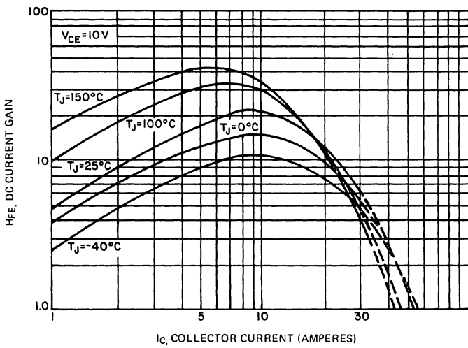
FIGURE 3. DC CURRENT GAIN ( V_{CE} = 10V )
