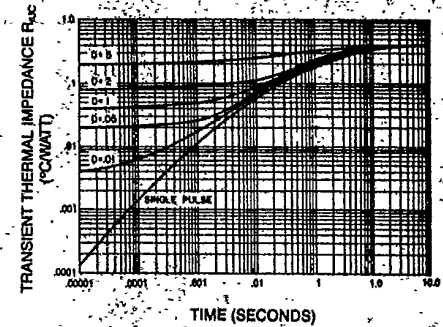
TRANSIENT THERMAL IMPEDANCE CHARACTERISTICS (TRANSISTOR)
