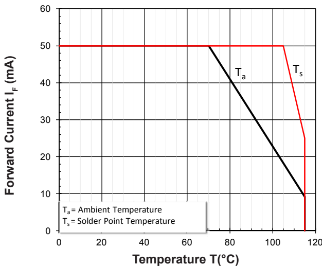
Maximum Current Vs Temperature (Red) I_F = f(T)
