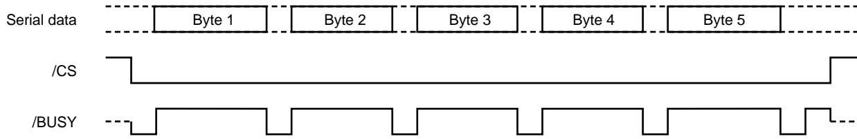
Figure 7-2. Inputting 5 Bytes Successively
